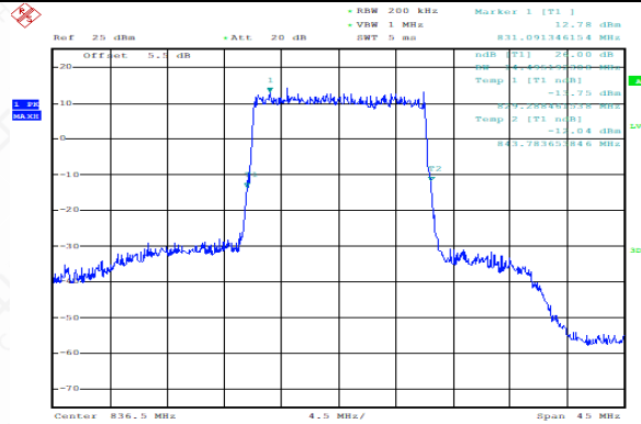
FDD26(PART 22)_Channel Mid_15MHz_836.5MHz_Q16
