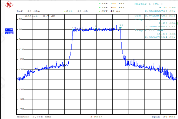
TDD40(2350-2360MHz)_Channel Mid_10_2355_Q16
