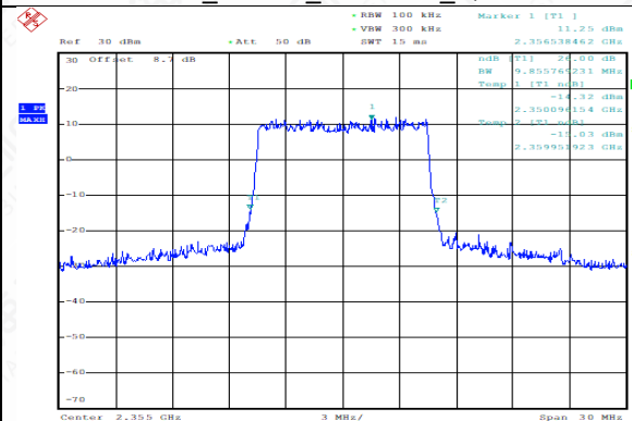
TDD40(2350-2360MHz)_Channel Mid_10MHz_2355MHz_Q16
