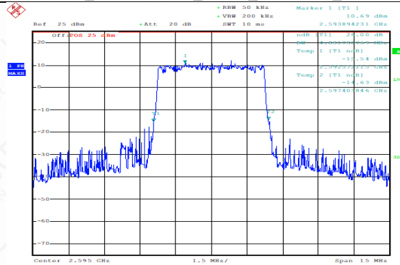
TDD38_Channel Mid_5MHz_2595MHz_Q16
