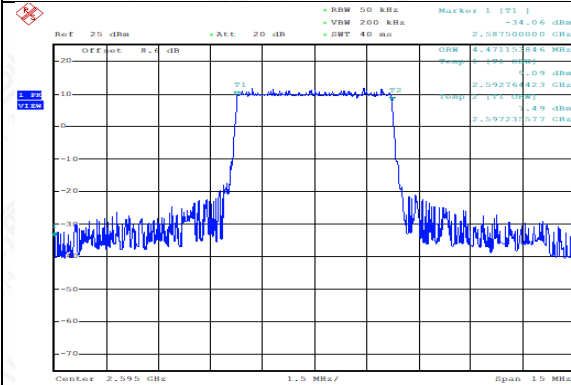
TDD38_Channel Mid_5_2595_QPSK
