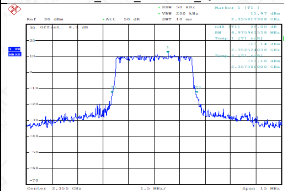
TDD40(2350-2360MHz)_Channel Mid_5MHz_2355MHz_Q16
