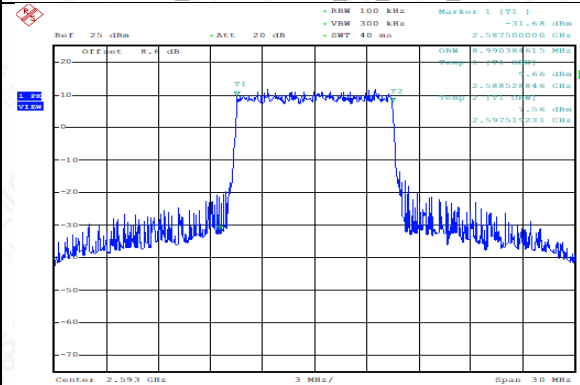
TDD41_Channel Mid_10_2593_Q16
