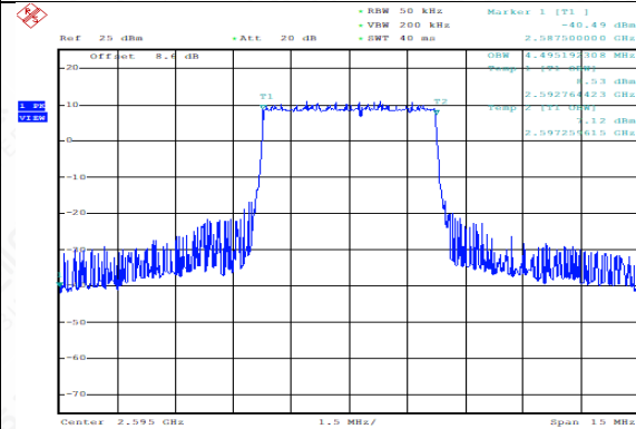
TDD38_Channel Mid_5_2595_Q16
