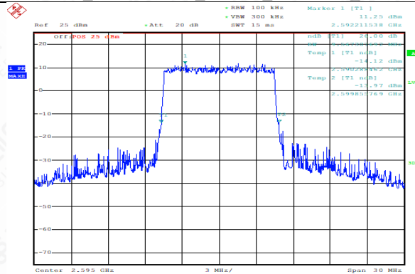
TDD38_Channel Mid_10MHz_2595MHz_Q16
