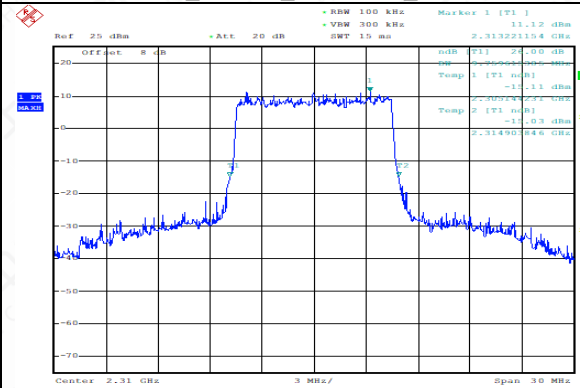
TDD40(2305-2315MHz)_Channel Mid_10MHz_2310MHz_Q16
