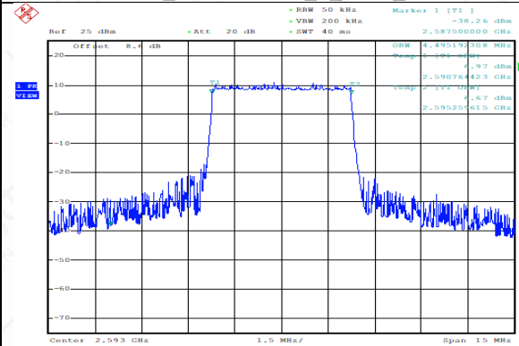
TDD41_Channel Mid_5_2593_Q16
