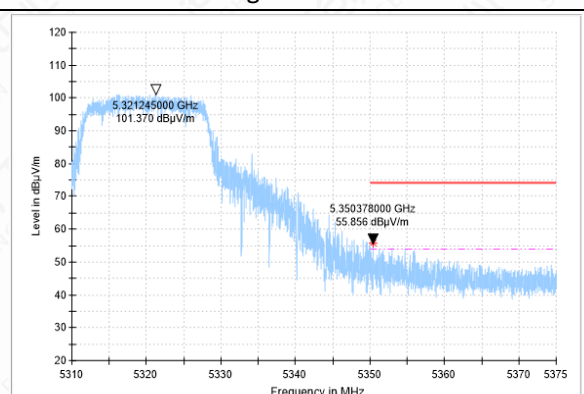
Bandedge-11A-CH64-PK
