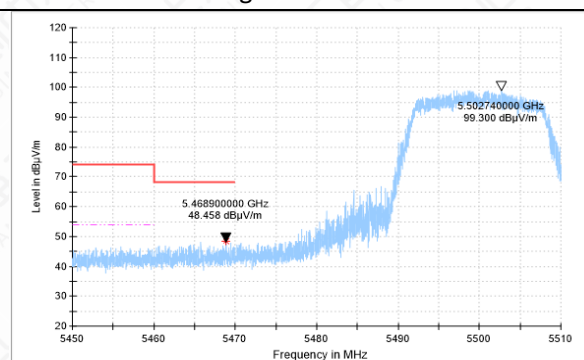
Bandedge-11A-CH100-PK
