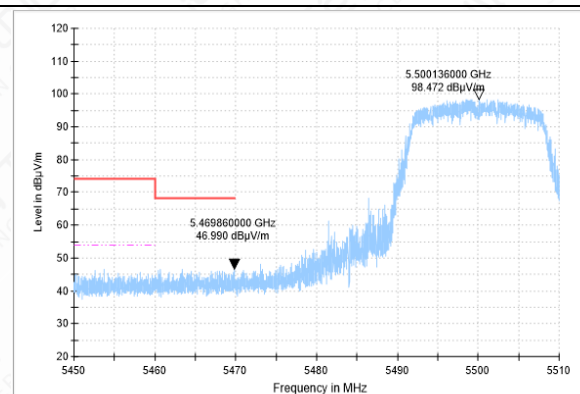
Bandedge-11A-CH100-PK
