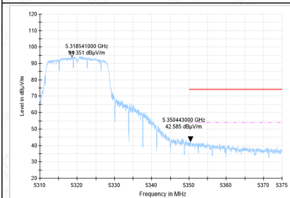
Bandedge-11A-CH64-AV
