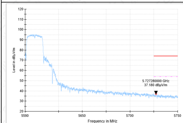
Bandedge-11A-CH120-AV
