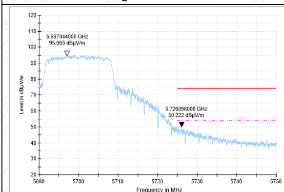
Bandedge-11A-CH140-AV
