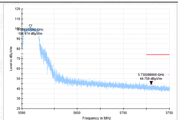
Bandedge-11A-CH120-PK
