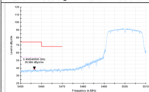
Bandedge-11A-CH100-AV
