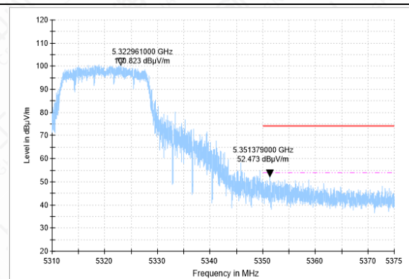
Bandedge-11A-CH64-PK
