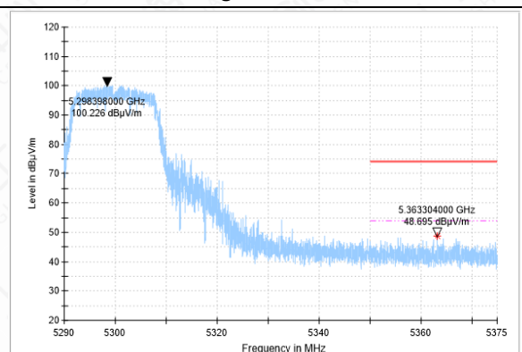
Bandedge-11A-CH60-PK
