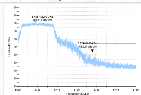
Bandedge-11A-CH140-PK
