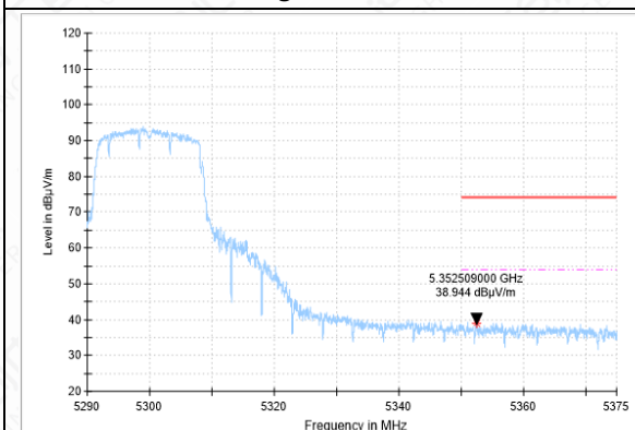
Bandedge-11A-CH60-AV
