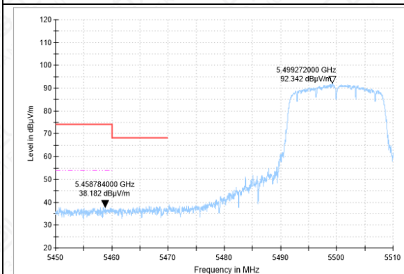
Bandedge-11A-CH100-AV
