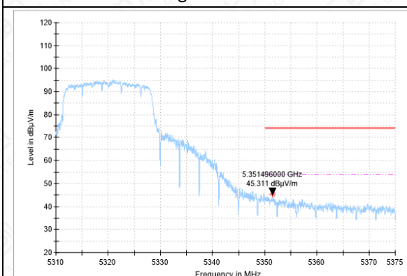
Bandedge-11A-CH64-AV
