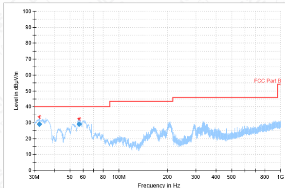
Radiated Spurious Emission (802.11a, ch120, 30MHz-1GHz)
