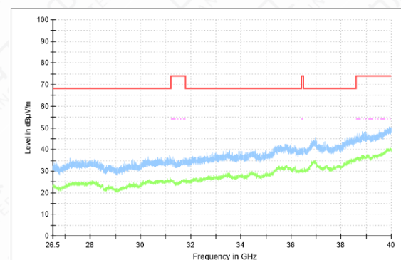
Radiated Spurious Emission (802.11a ch120, 26.5GHz-40GHz)
