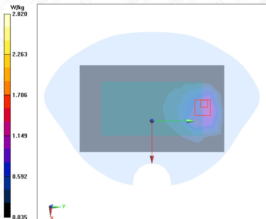
Figure A.1-2 LTE B12 10MHz 1RB 25offset Front Mode Low 0mm
