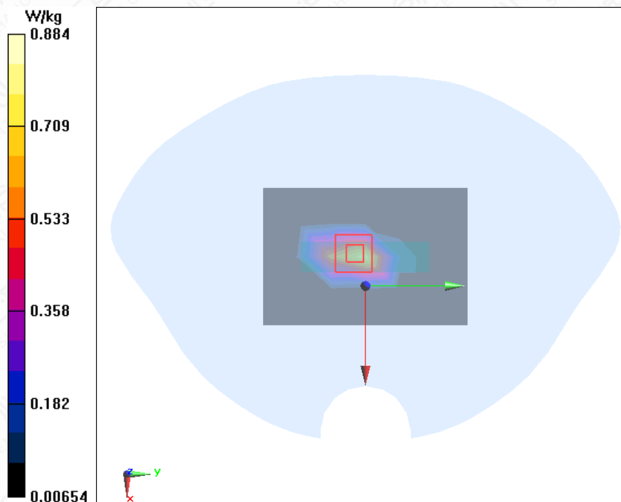
Figure A.1-3 LTE B25 20MHz 1RB 50offset Bottom Mode High 5mm
