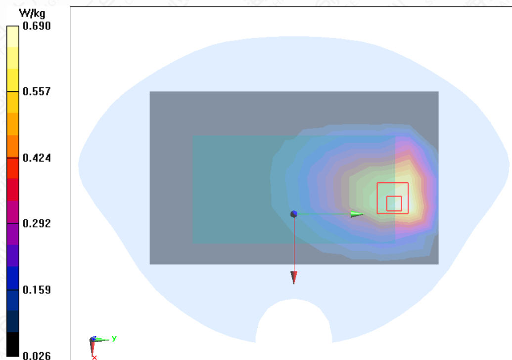
Figure A.1-5 LTE B26 15MHz 1RB 38offset Front Mode Middle 5mm
