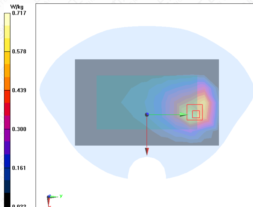
Figure A.1-1 LTE B12 10MHz 1RB 25offset Front Mode High 5mm
