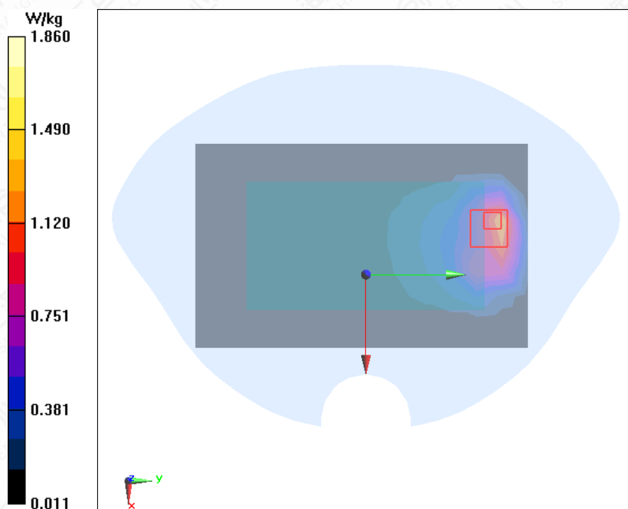
Figure A.1-6 LTE B26 15MHz 1RB 38offset Front Mode Middle 0mm
