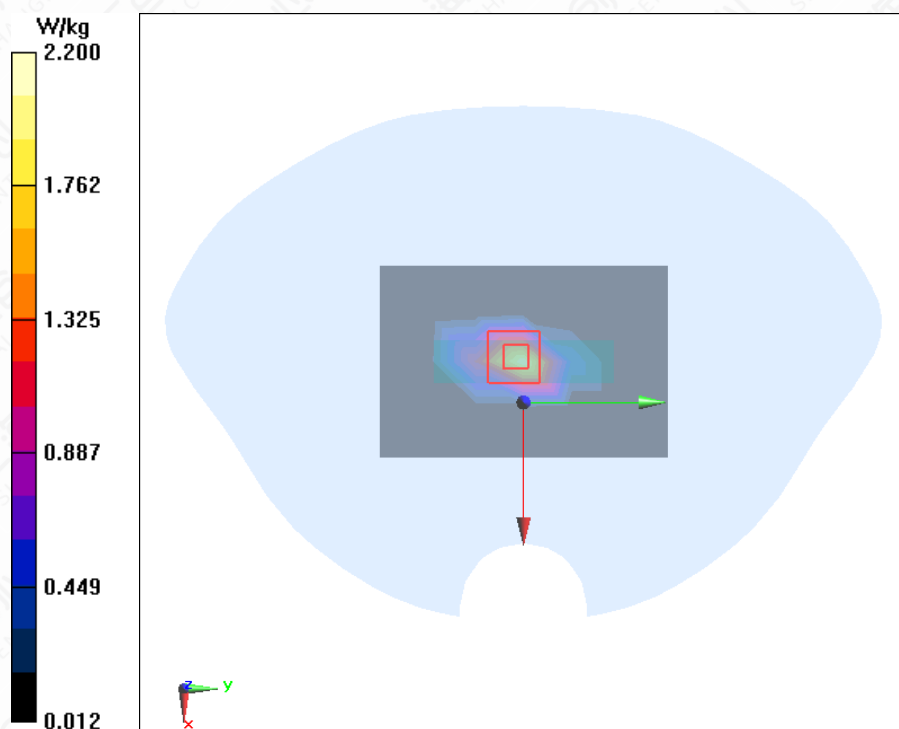
Figure A.1-4 LTE B25 20MHz 1RB 50offset Bottom Mode High 0mm
