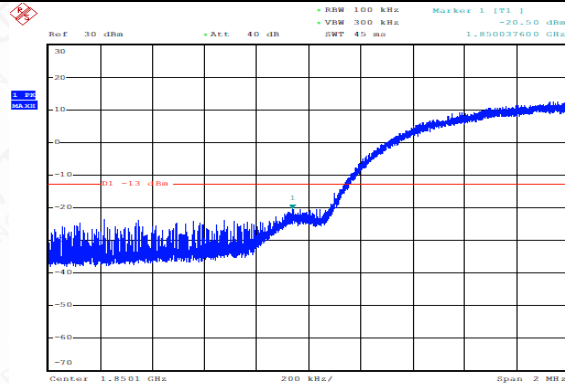
WCDMA_OB2,1852.6MHz_BandEdge
