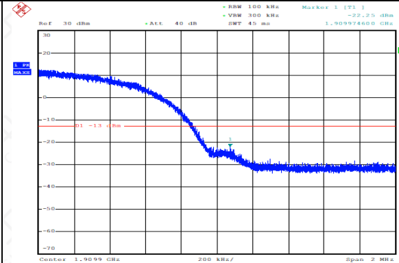
WCDMA_OB2,1907.4MHz_BandEdge
