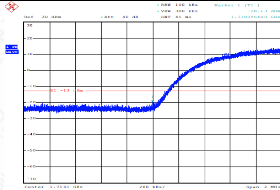
WCDMA_OB4,1712.6MHz_BandEdge
