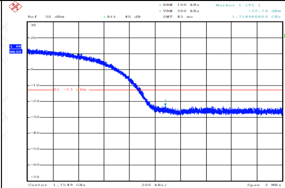
WCDMA_OB4,1752.4MHz_BandEdge
