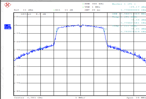
99% Occupied Bandwidth ( MHz) (802.11n-HT20, 5785MHz)
