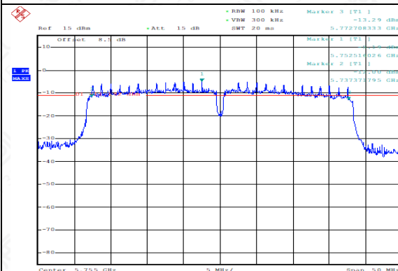
Occupied 6dB Bandwidth ( MHz) (802.11n-HT40, 5755MHz)
