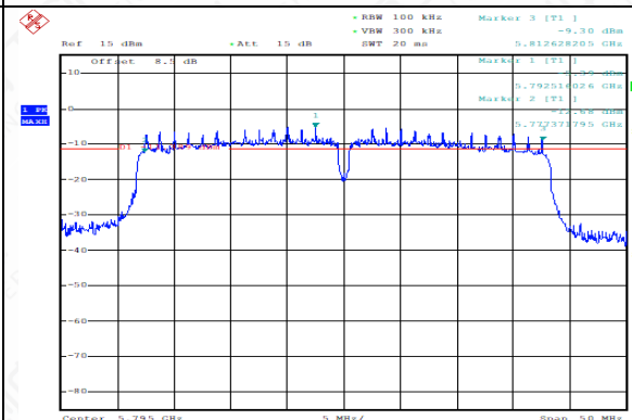
Occupied 6dB Bandwidth ( MHz) (802.11n-HT40, 5795MHz)
