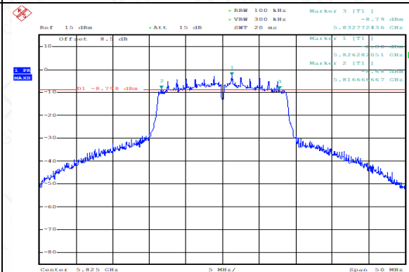
Occupied 6dB Bandwidth ( MHz) (802.11n-HT20, 5825MHz)
