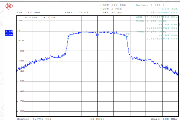
99% Occupied Bandwidth ( MHz) (802.11n-HT40, 5795MHz)
