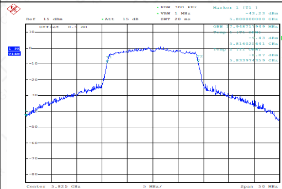
99% Occupied Bandwidth ( MHz) (802.11n-HT20, 5825MHz)
