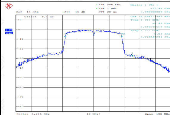
99% Occupied Bandwidth ( MHz) (802.11n-HT40, 5755MHz)
