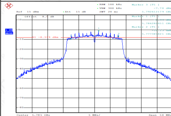
Occupied 6dB Bandwidth ( MHz) (802.11n-HT20, 5785MHz)
