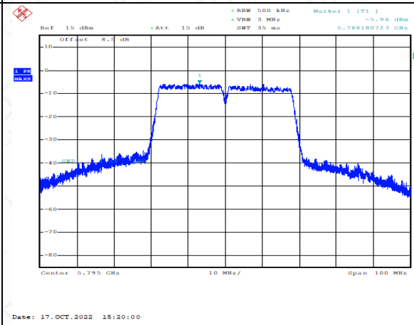
Power Spectral Density(dBm/500kHz) (802.11n- HT40), 5795MHz)
