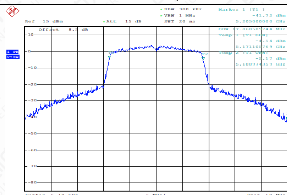
99% Occupied Bandwidth (MHz) (802.11n-HT20), 5180MHz)
