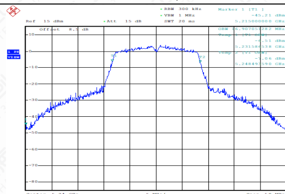
99% Occupied Bandwidth (MHz) (802.11a, 5240MHz)
