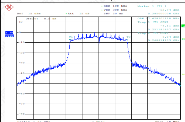
99% Occupied Bandwidth (MHz) (802.11n-HT20), 5260MHz)
