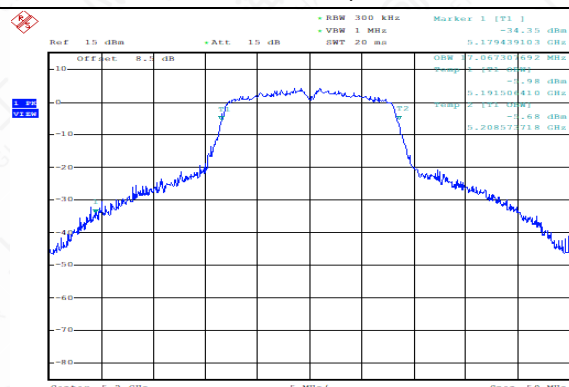
99% Occupied Bandwidth (MHz) (802.11a, 5200MHz)
