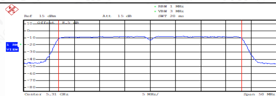
Output Power-Conducted (802.11n-HT40, Ch62)
