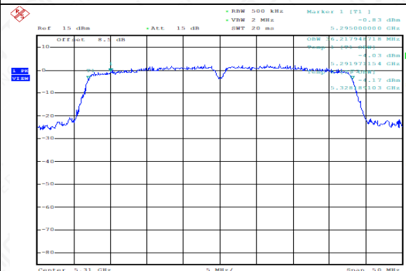
99% Occupied Bandwidth (MHz) (802.11n-HT40), 5310MHz)
