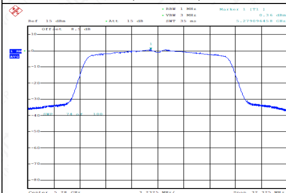
Power Spectral Density(dBm/MHz) (802.11n-HT20), 5280MHz)
