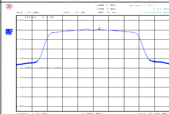
Power Spectral Density(dBm/MHz) (802.11n-HT20), 5320MHz)
