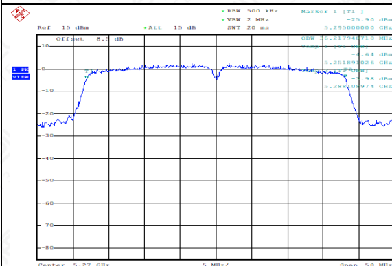
99% Occupied Bandwidth (MHz) (802.11n-HT40), 5270MHz)
