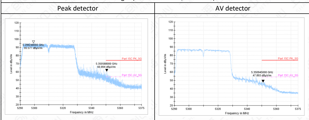
Band Edges (802.11n-40MHz, 5310MHz)
