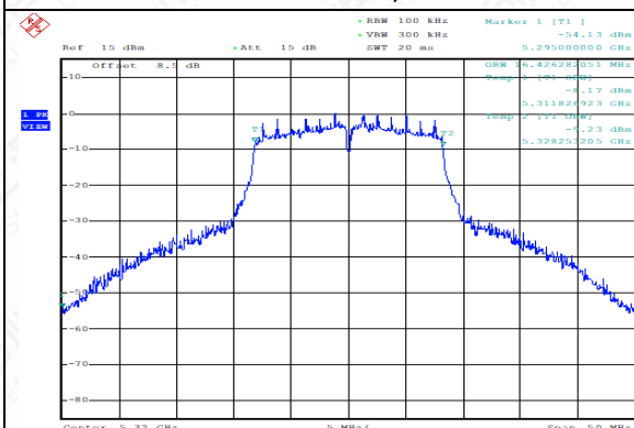
99% Occupied Bandwidth (MHz) (802.11a, 5320MHz)
