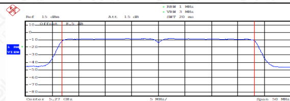
Output Power-Conducted (802.11n-HT40, Ch54)
