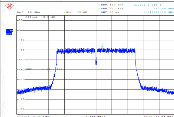
Power Spectral Density(dBm/MHz) (802.11n-HT40), 5310MHz)
