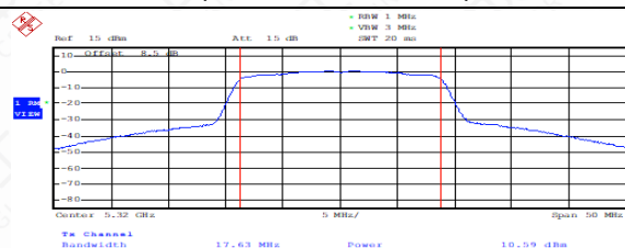
Output Power-Conducted (802.11n-HT20, Ch64)
