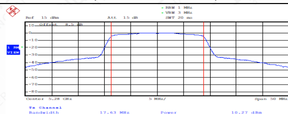
Output Power-Conducted (802.11n-HT20, Ch56)
