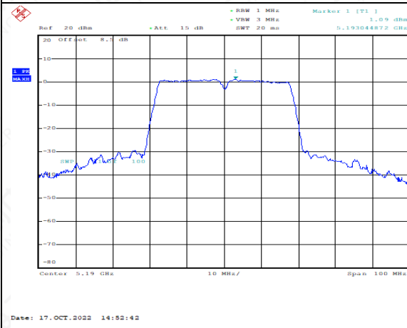
Power Spectral Density(dBm/MHz) (802.11n-HT40), 5190MHz)
