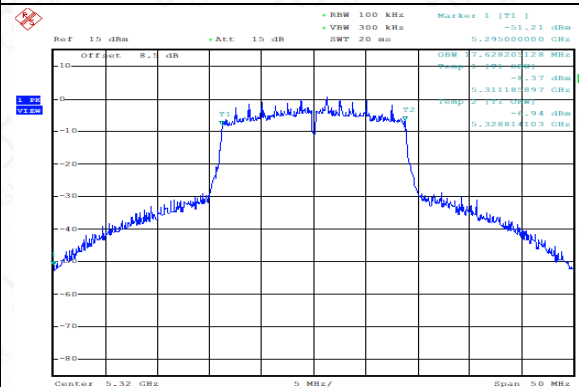
99% Occupied Bandwidth (MHz) (802.11n-HT20), 5320MHz)
