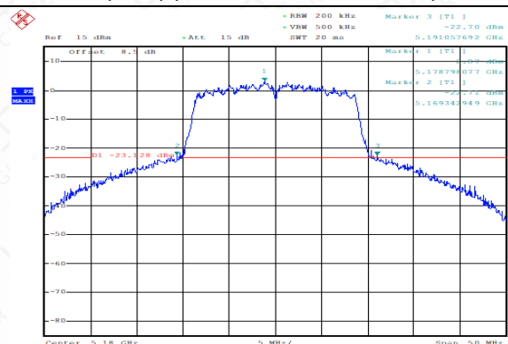
Occupied 26dB Bandwidth (MHz) (802.11n-HT20, 5180MHz)
