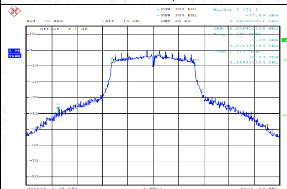
99% Occupied Bandwidth (MHz) (802.11a, 5280MHz)
