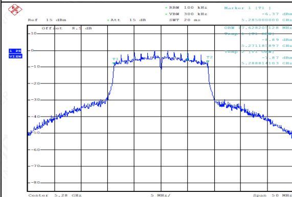
99% Occupied Bandwidth (MHz) (802.11n-HT20), 5280MHz)
