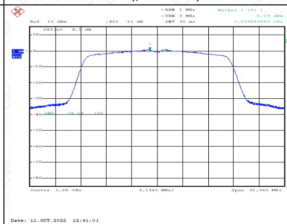
Power Spectral Density(dBm/MHz) (802.11n-HT20), 5260MHz)
