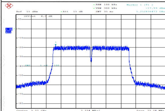
Power Spectral Density(dBm/MHz) (802.11n-HT40), 5270MHz)
