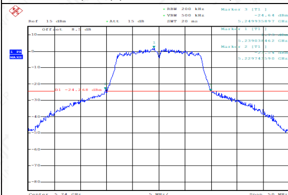
Occupied 26dB Bandwidth (MHz) (802.11a, 5240MHz)
