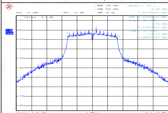
99% Occupied Bandwidth (MHz) (802.11a, 5260MHz)
