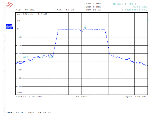
Power Spectral Density(dBm/MHz) (802.11n-HT40), 5230MHz)
