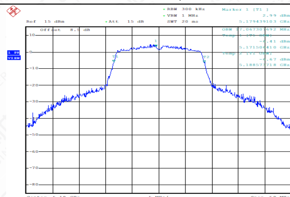
99% Occupied Bandwidth (MHz) (802.11a, 5180MHz)
