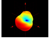
LTE12/L17(Frequency=740MHz)
