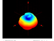
LTE28(Frequency=780MHz)
