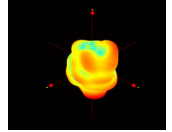
LTE5/G850/W5(Frequency=880MHz)
