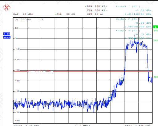
Band Edges (802.11n-20MHz, Ch1)
