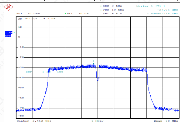
Power Spectral Density (802.11n-40MHz, Ch9)
