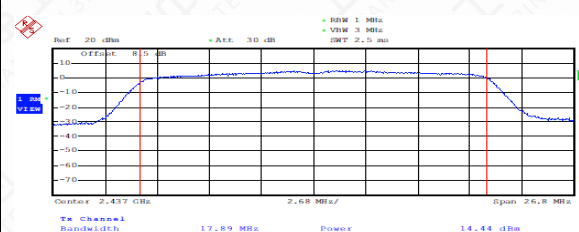
Output Power-Conducted (802.11n-20MHz, Ch6)
