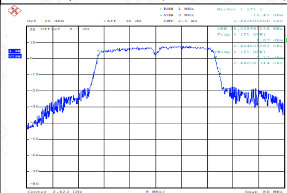
99% Occupied Bandwidth (802.11n-40MHz, Ch3)
