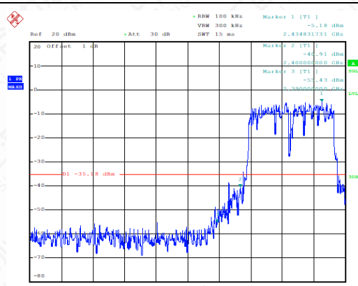
Band Edges (802.11n-40MHz, Ch3)
