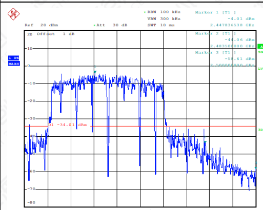
Band Edges (802.11n-40MHz, Ch9)
