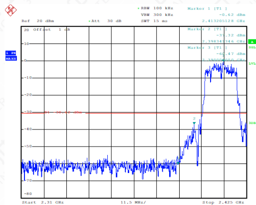
Band Edges (802.11g, Ch1)
