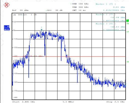
Band Edges (802.11g, Ch11)
