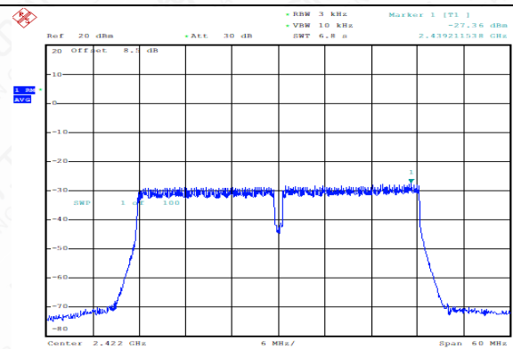
Power Spectral Density (802.11n-40MHz, Ch3)
