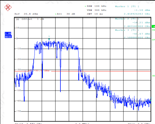
Band Edges (802.11n-20MHz, Ch11)
