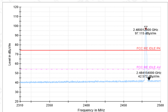
Bandedge (High): GFSK, high channel
