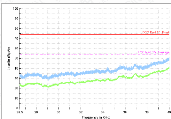
Radiated emission: GFSK, Ch78, 26.5GHz~40GHz
