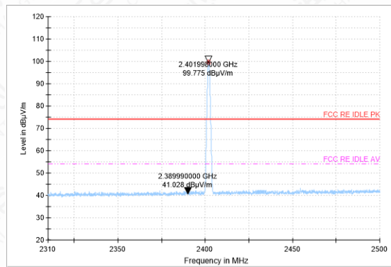
Bandedge (Low): GFSK, low channel
