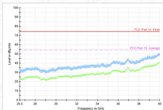
Radiated emission: GFSK, Ch0, 26.5GHz~40GHz
