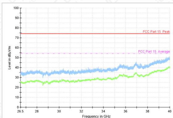
Radiated emission: GFSK, Ch0, 26.5GHz~40GHz
