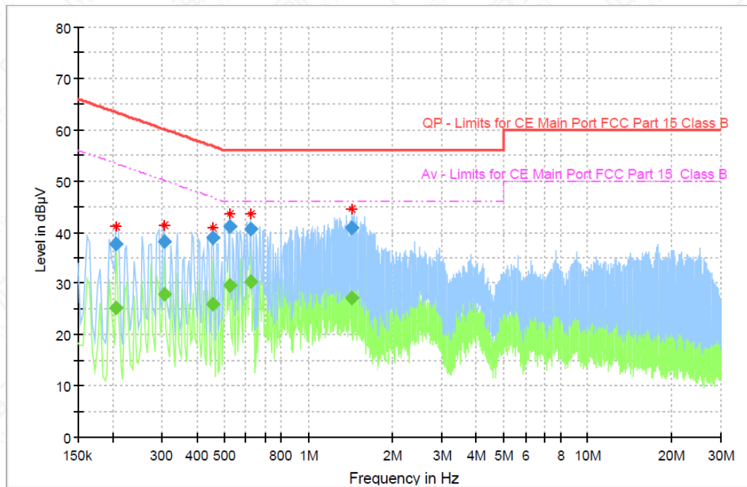
Figure A.2-2 Mode 8 (150kHz-30MHz) _ S16aa (Fingerprint edition secondary supply) + BB02
