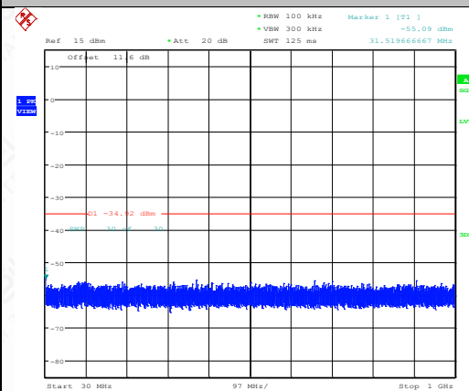
11N40SISO-Ant1-2437-30~1000-PASS
