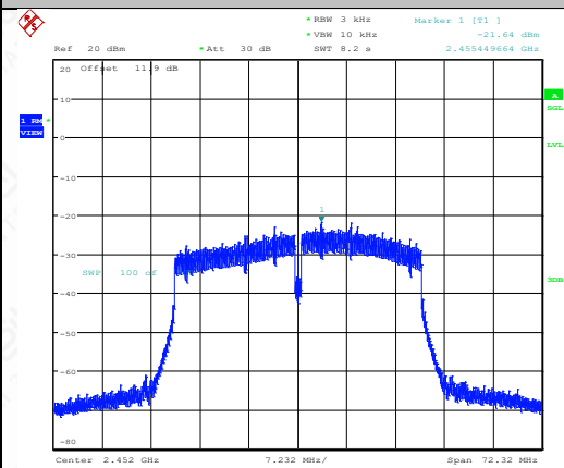
11N40SISO-Ant1-2452-PASS
