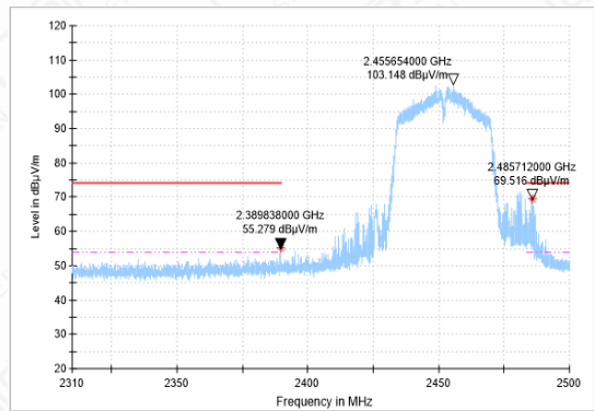
BANDEDGE-11N(40M)-CH9-PK
