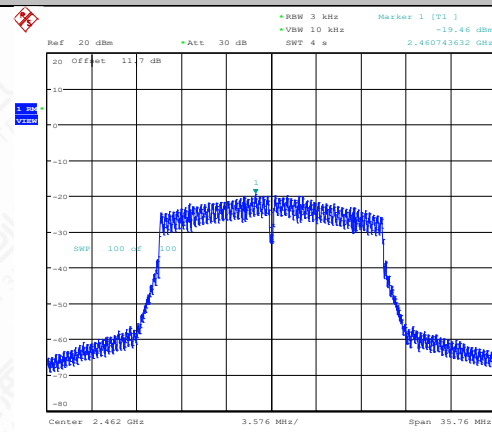
11N20SISO-Ant1-2462-PASS
