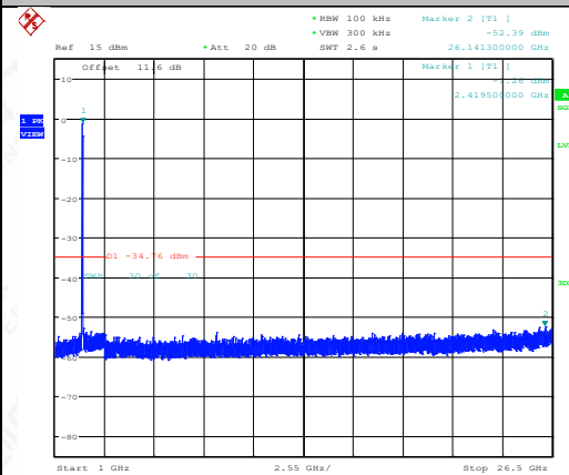
11N40SISO-Ant1-2422-1000~26500-PASS
