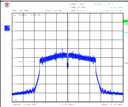
11N40SISO-Ant1-2422-PASS
