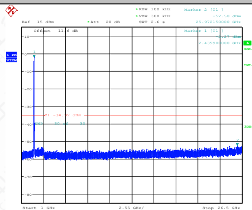
11N40SISO-Ant1-2437-1000~26500-PASS
