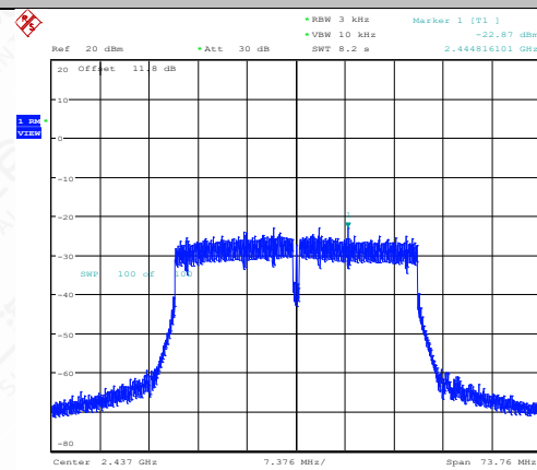
11N40SISO-Ant1-2437-PASS
