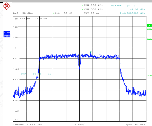
11N40SISO-Ant1-2437-0~Reference-PASS
