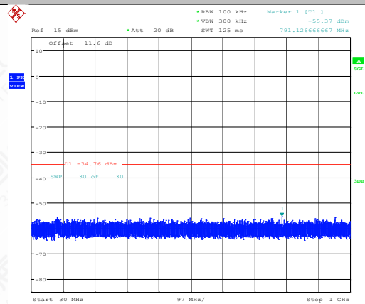
11N40SISO-Ant1-2422-30~1000-PASS
