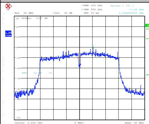
11N40SISO-Ant1-2452-0~Reference-PASS
