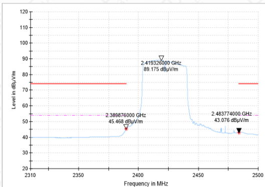
BANDEDGE-11N(40M)-CH3-AV
