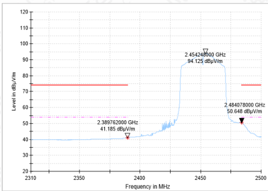
BANDEDGE-11N(40M)-CH9-AV
