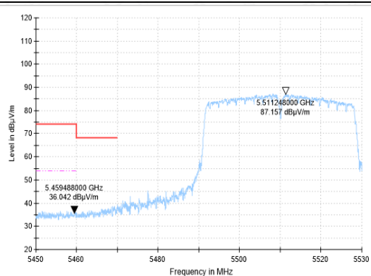
BANDEGE-11N(40M)-CH102-AV-13
