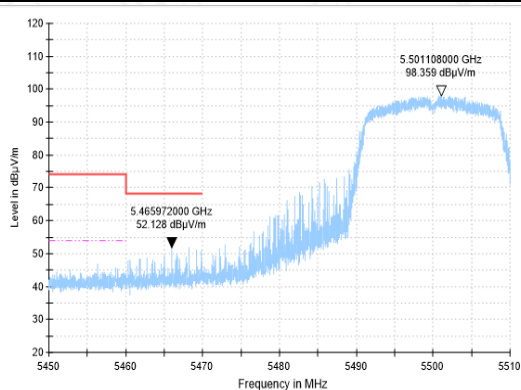
BADEDGE-11N-CH100-PK
