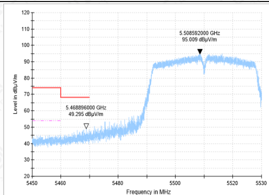
BANDEGE-11AC(40M)-CH102-PK
