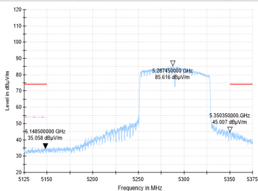
BANDEDGE-11AC(80M)-CH58-AV-11
