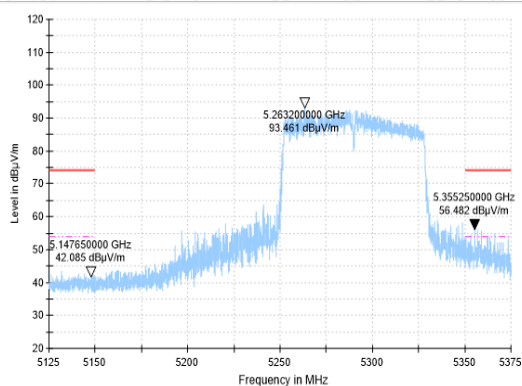
BANDEDGE-11AC(80M)-CH58-PK-11
