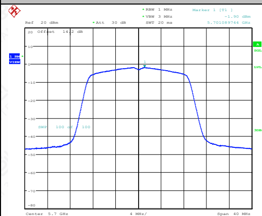
11N20SISO-Ant1-5700-PASS
