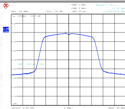
11N20SISO-Ant1-5580-PASS
