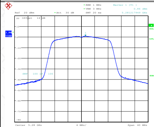
11N20SISO-Ant1-5280-PASS
