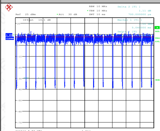
NTNV-11AC40SISO-Ant1-5670
