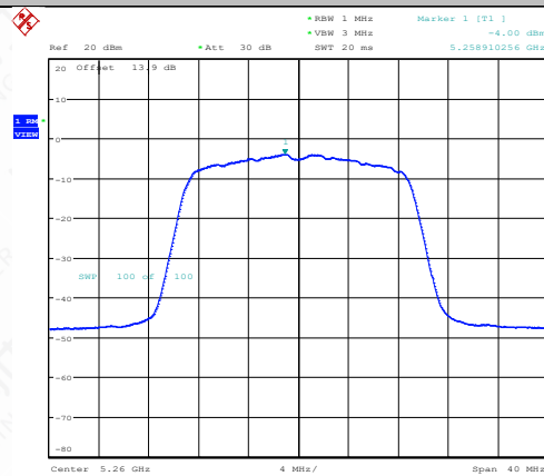
11N20SISO-Ant1-5260-PASS
