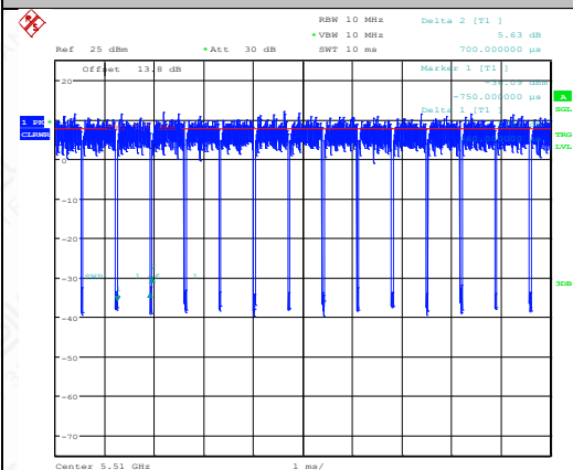
NTNV-11AC40SISO-Ant1-5510
