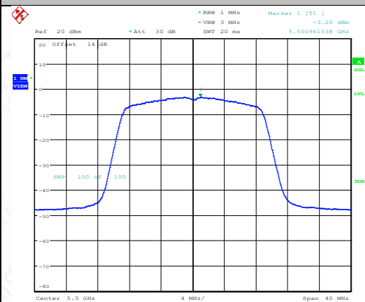
11N20SISO-Ant1-5500-PASS
