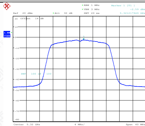
11N20SISO-Ant1-5320-PASS
