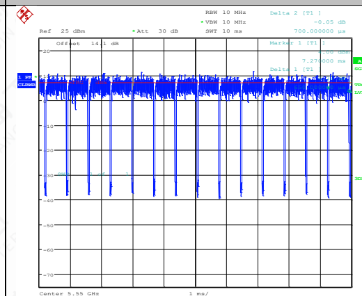
NTNV-11AC40SISO-Ant1-5550
