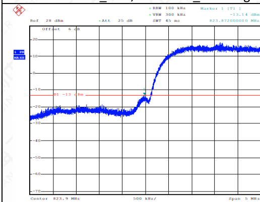
WCDMA_OB5,826.4MHz_BandEdge
