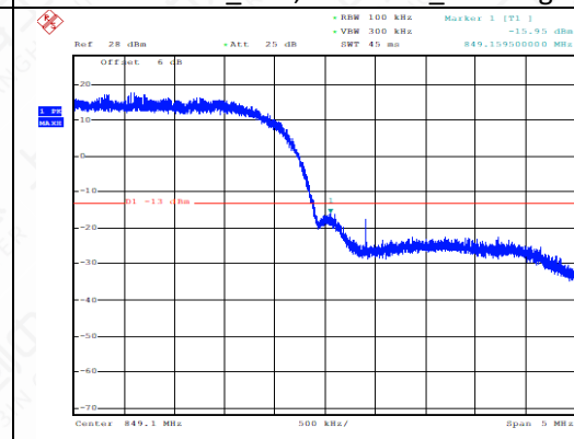
WCDMA_OB5,846.6MHz_BandEdge
