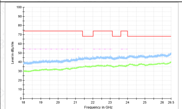
RSE-11N(40M)-CH159-18GHz-26.5GHz
