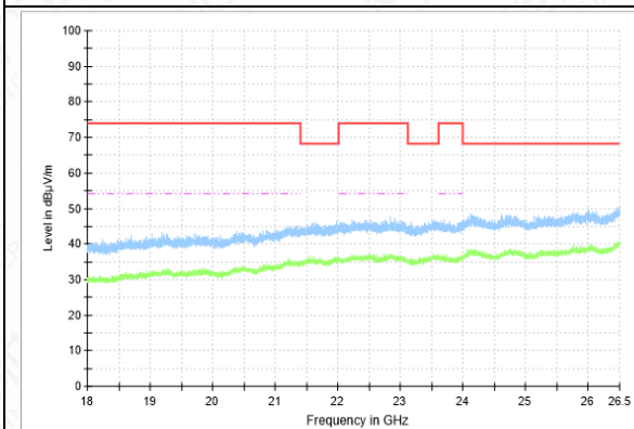
RSE-11AC(80M)-CH155-18GHz-26.5GHz
