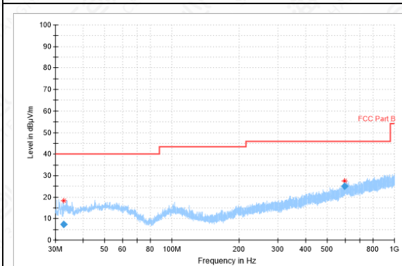
RSE-11N(40M)-CH159-30MHz-1GHz
