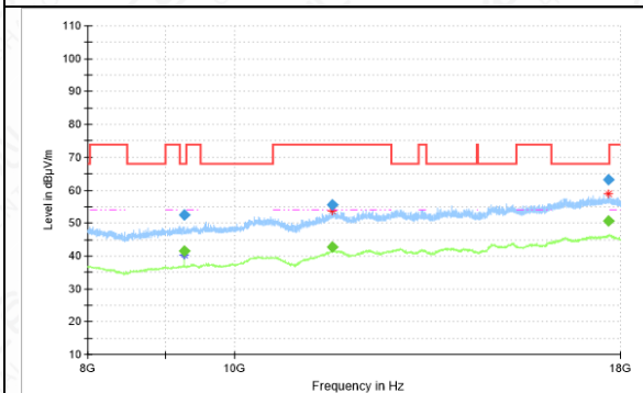
RSE-11N(40M)-CH159-8GHz-18GHz
