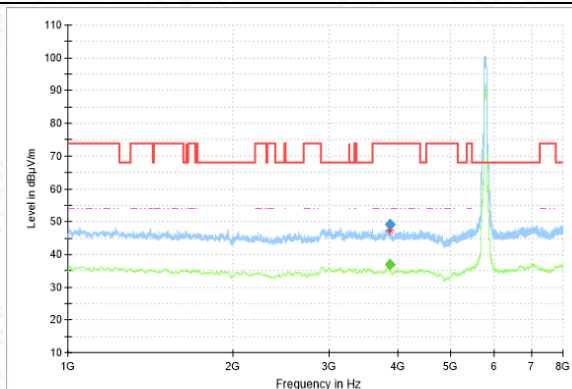
RSE-11AC(80M)-CH155-1GHz-8GHz
