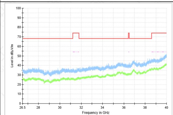
RSE-11AC(80M)-CH155-26.5GHz-40GHz
