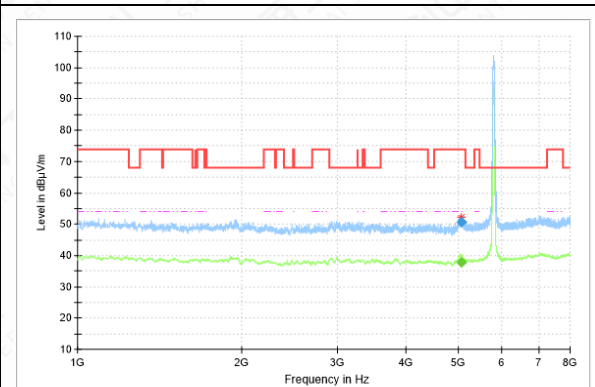
RSE-11N(40M)-CH159-1GHz-8GHz
