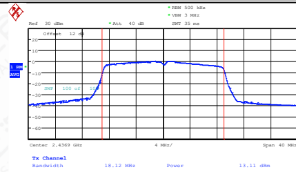
11N20SISO-Ant1-2437-PASS
