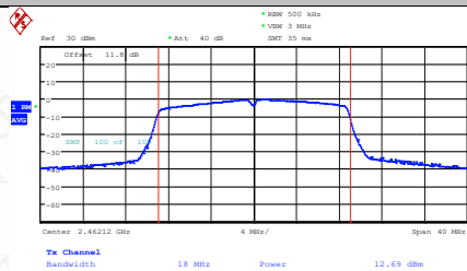
11N20SISO-Ant1-2462-PASS
