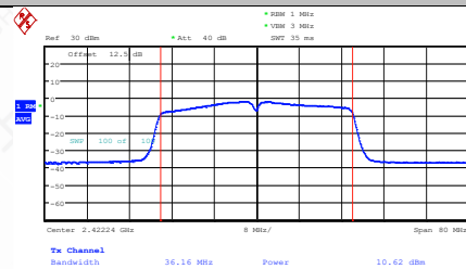
11N40SISO-Ant1-2422-PASS
