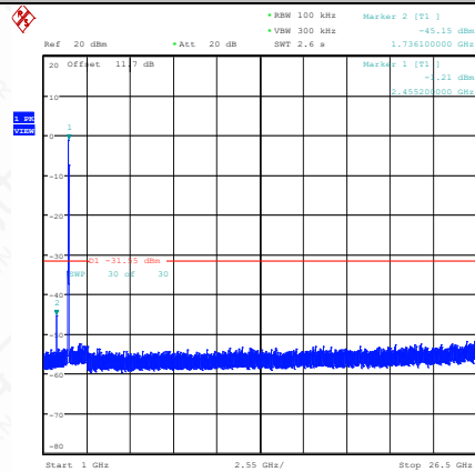
11N40SISO-Ant1-2452-1000~26500-PASS
