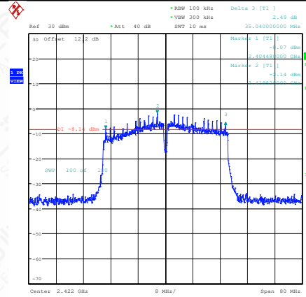
11N40SISO-Ant1-2422-PASS
