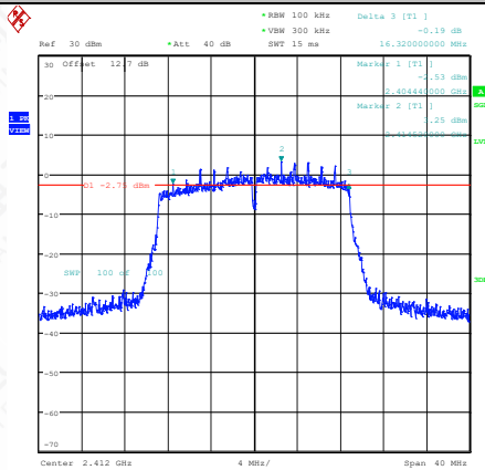
11N20SISO-Ant1-2412-PASS
