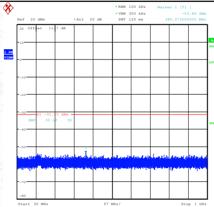
11N40SISO-Ant1-2452-30~1000-PASS
