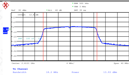
11N20SISO-Ant1-2412-PASS
