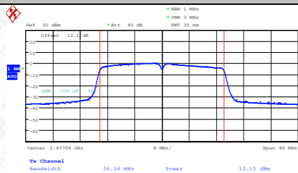
11N40SISO-Ant1-2437-PASS
