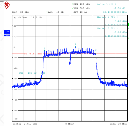
11N40SISO-Ant1-2452-PASS
