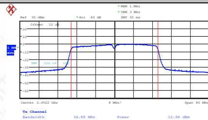
11N40SISO-Ant1-2452-PASS
