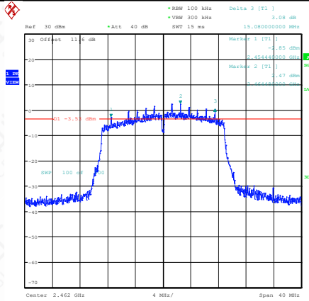
11N20SISO-Ant1-2462-PASS
