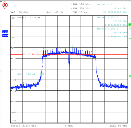
11N40SISO-Ant1-2437-PASS
