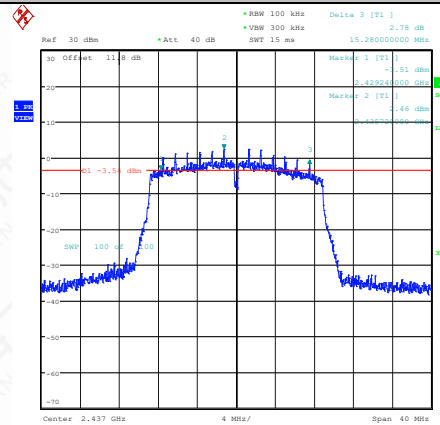
11N20SISO-Ant1-2437-PASS
