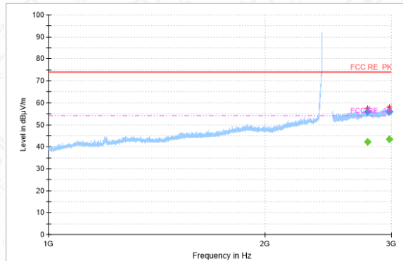
RSE-11N(20M)-CH1-1GHz-3GHz
