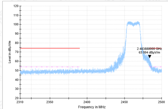
Bandedge-11N(20M)-CH11-PK
