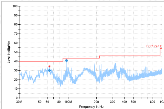
RSE-11N(20M)-CH1-30MHz-1GHz
