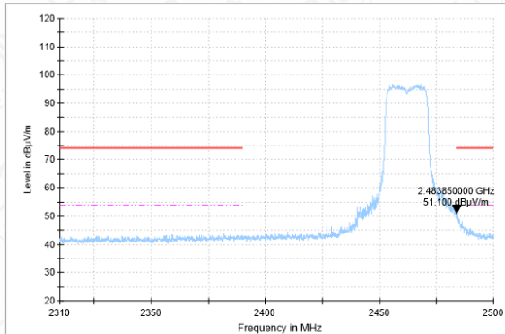
Bandedge-11N(20M)-CH11-AV
