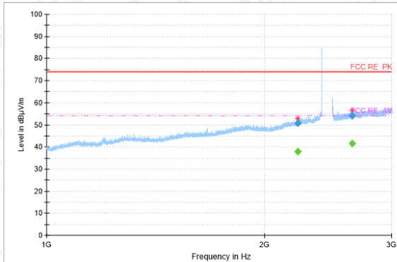
RSE-11G-CH11-1GHz-3GHz
