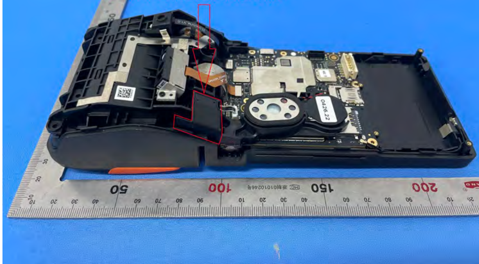
WWAN Main Antenna
