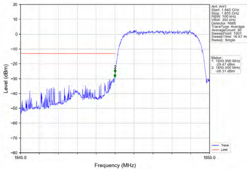
Band2 HSDPA LCH 1852.4MHz Subtest 1 NTN
