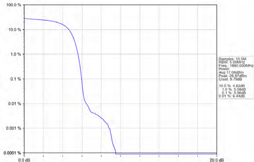
Band2 HSUPA MCH 1880MHz Subtest 1 NTN
