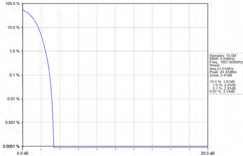
Band2 RMC HCH 1907.6MHz 12.2kbps RMC NTN
