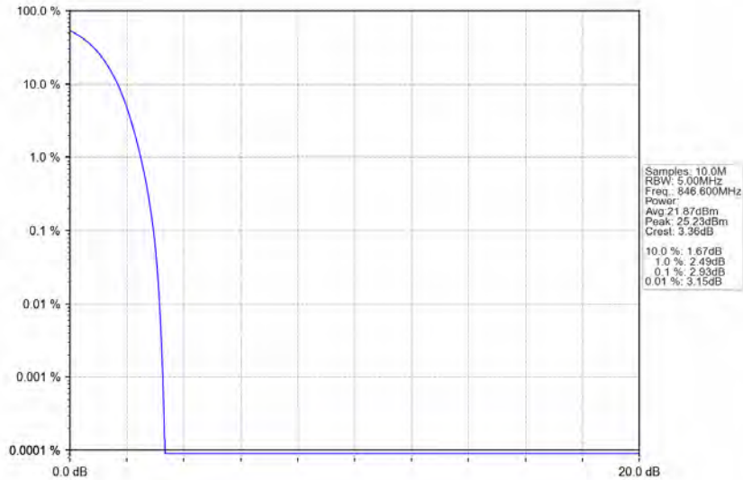
Band5_RMC_HCH_846.6MHz_12.2kbps_RMC_NTNV
