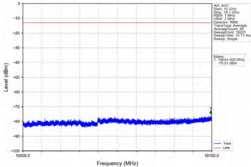
Band2 HSDPA MCH 1880MHz Subtest 1 NTN
