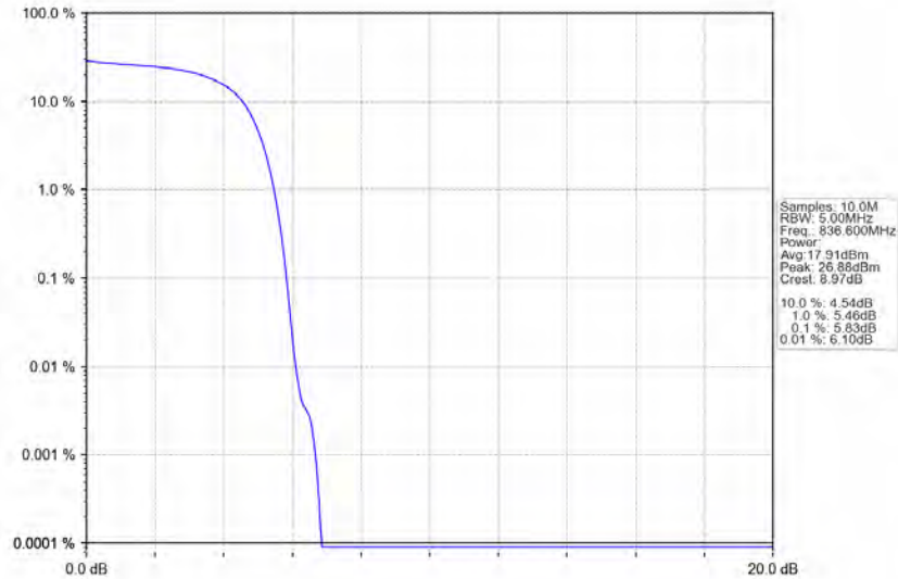
Band5 HSDPA MCH 836.6MHz Subtest 1 NTN
