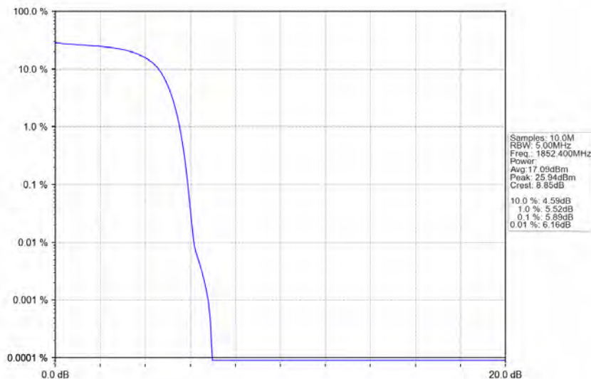
Band2 HSDPA LCH 1852.4MHz Subtest 1 NTN
