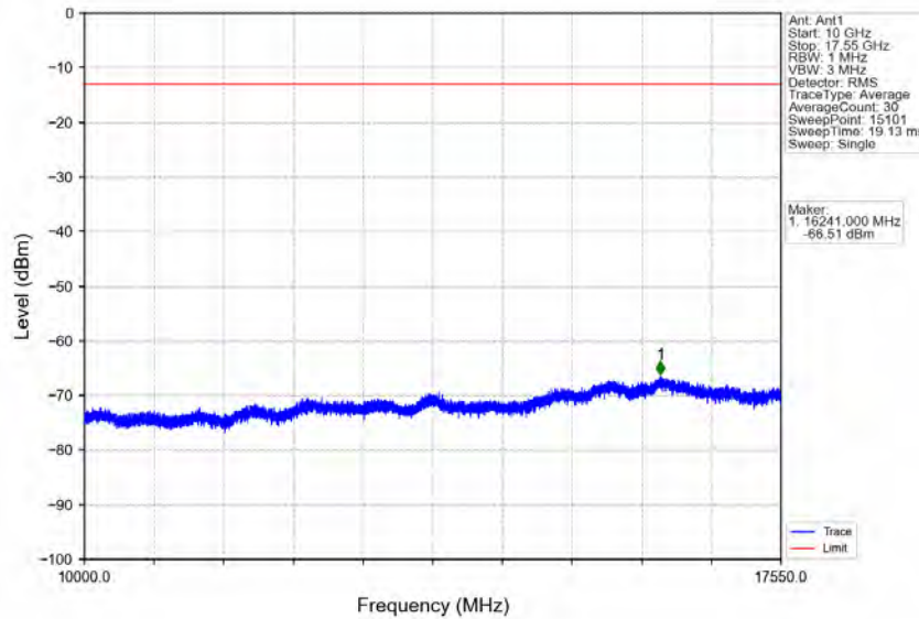
Band4 HSDPA MCH 1732.6MHz Subtest 1 NTN
