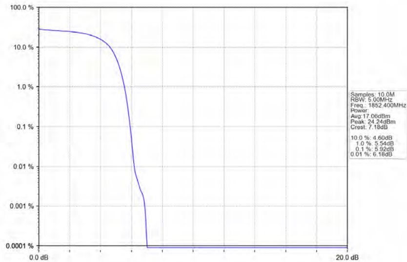
Band2 HSUPA LCH 1852.4MHz Subtest 1 NTN
