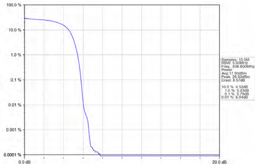
Band5 HSUPA MCH 836.6MHz Subtest 1 NTN
