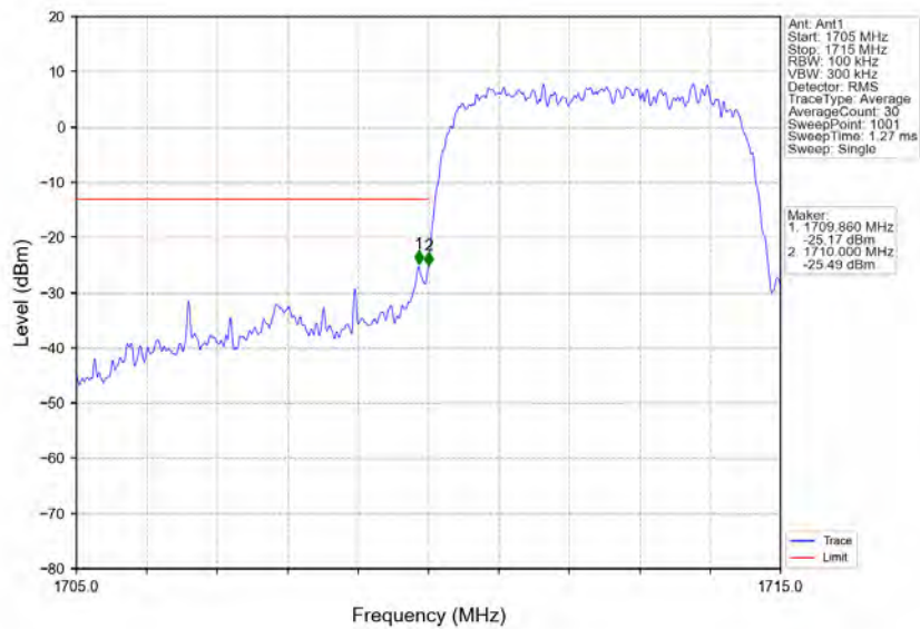
Band4 HSDPA LCH 1712.4MHz Subtest 1 NTN
