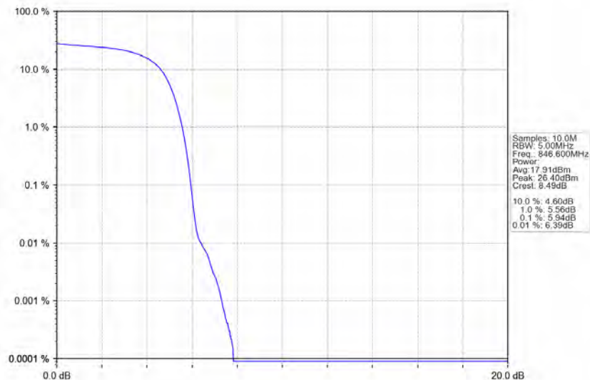
Band5 HSDPA HCH 846.6MHz Subtest 1 NTN
