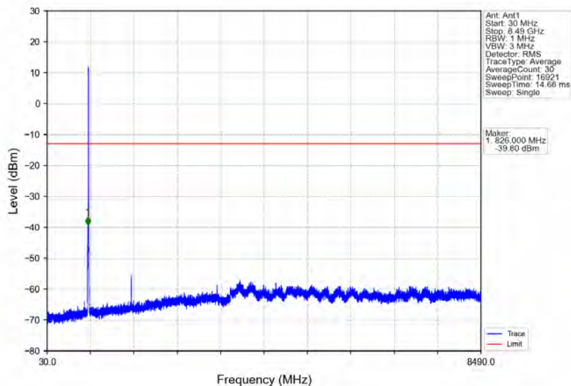
Band5 HSDPA MCH 836.6MHz Subtest 1 NTN
