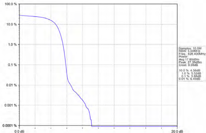
Band5_HSDPA_LCH_826.4MHz_Subtest 1_NTNV
