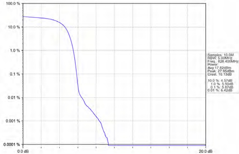
Band5 HSUPA LCH 826.4MHz Subtest 1 NTN
