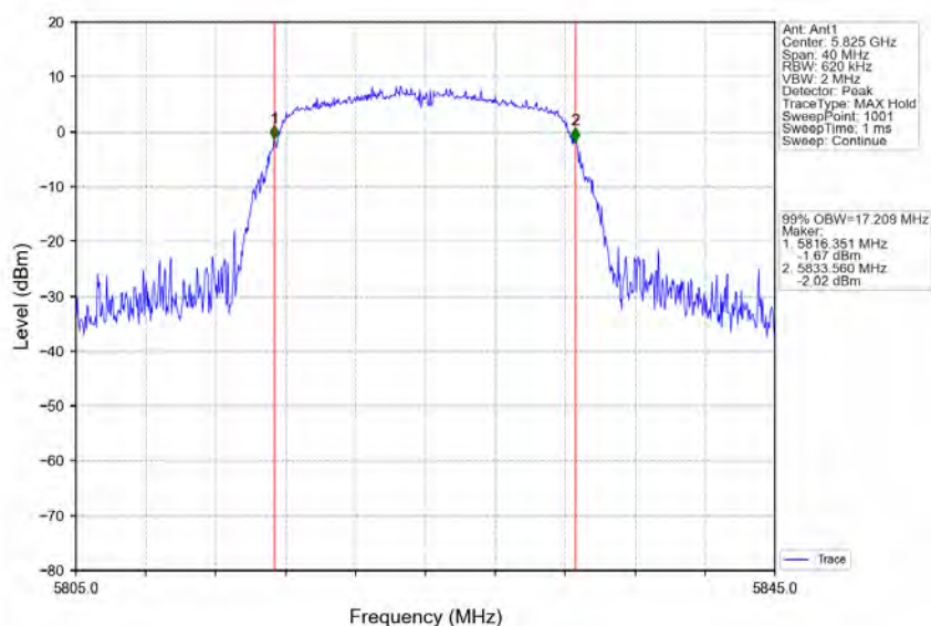
802.11a_HCH_5825MHz_Ant1_NTNV
