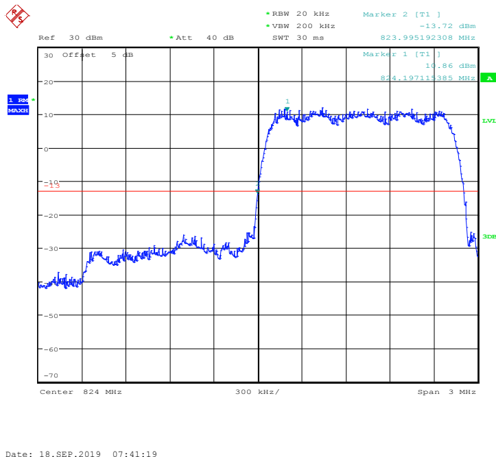
Fig.25 Channel 1013- LOW BAND EDGE BLOCK
