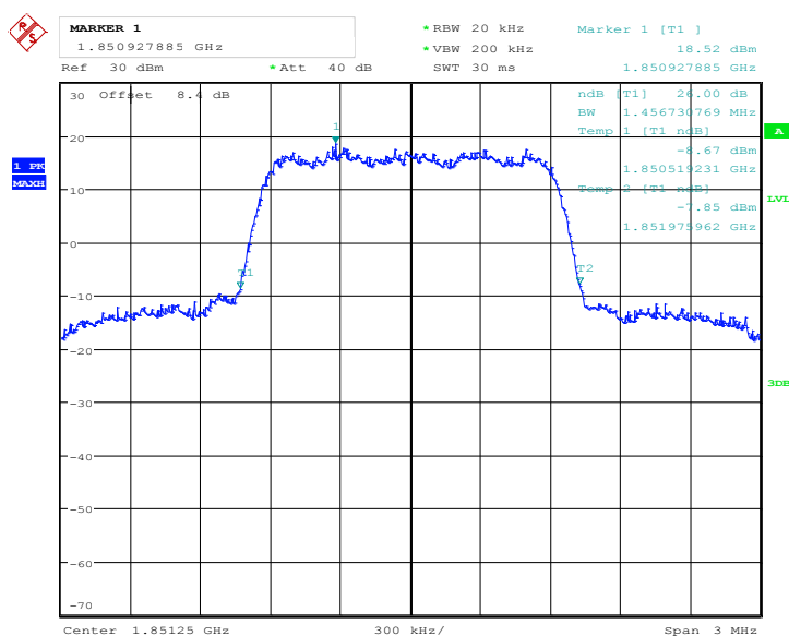
Fig.16 Channel 600- Emission Bandwidth (-26dBc BW)
