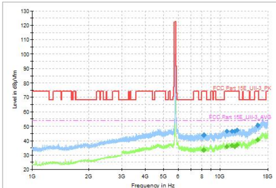
Fig. 60 Transmitter Spurious Emission (802.11ac-VHT40, CH159 5795MHz, 1GHz-18GHz)
