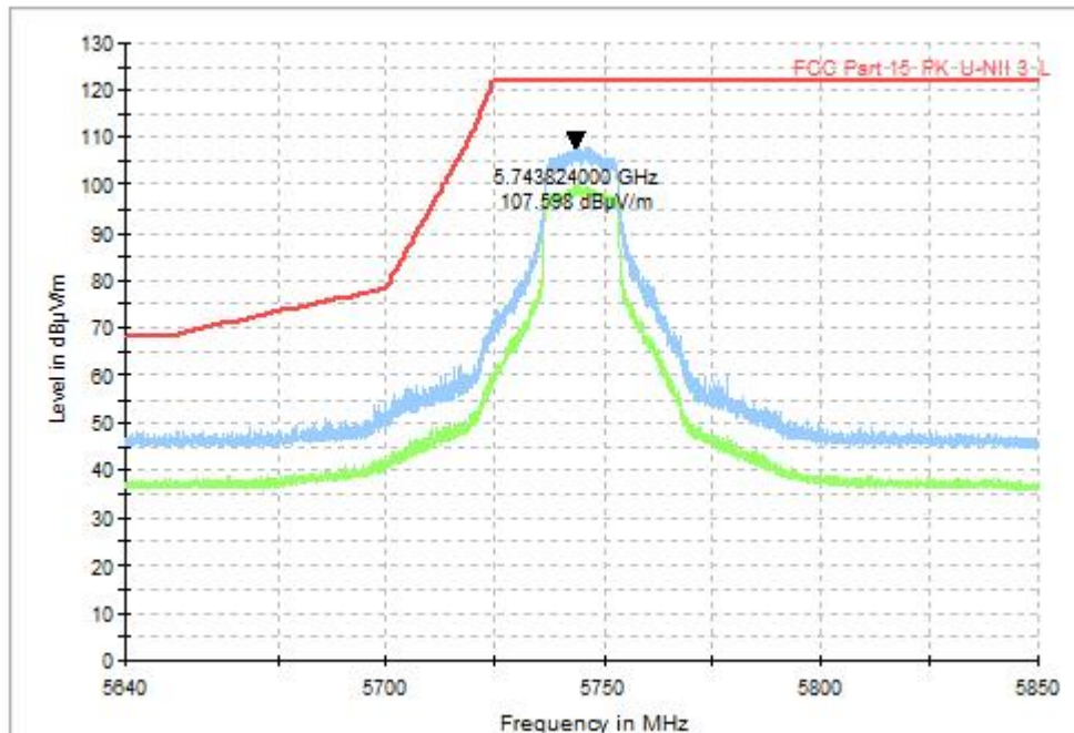
Fig. 27 Band Edges (802.11a, CH149 5745MHz)
