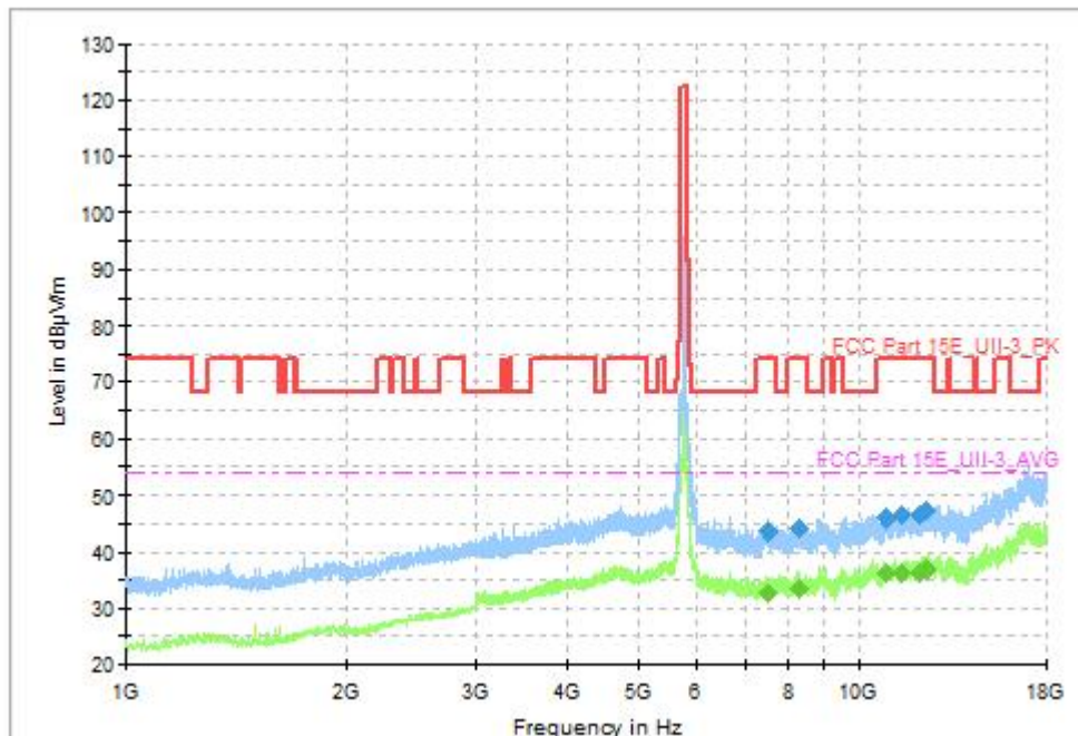
Fig. 65 Transmitter Spurious Emission (802.11ac-VHT80, CH155 5775MHz, 1GHz-18GHz)
