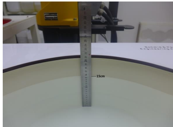
Photo 6: Tissue Simulant Liquid for Head 2300
