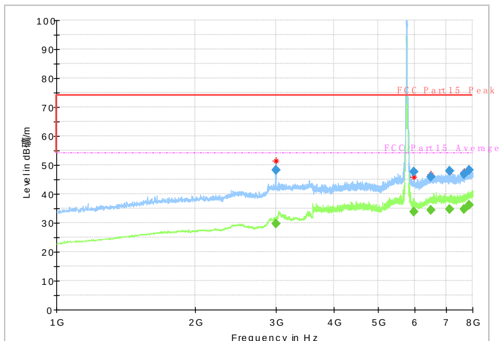
Fig. 37 Radiated Spurious Emission (802.11n-HT40, Ch151, 1 GHz-8 GHz)
