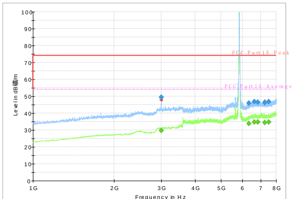
Fig. 27 Radiated Spurious Emission (802.11a, Ch165, 1 GHz-8 GHz)
