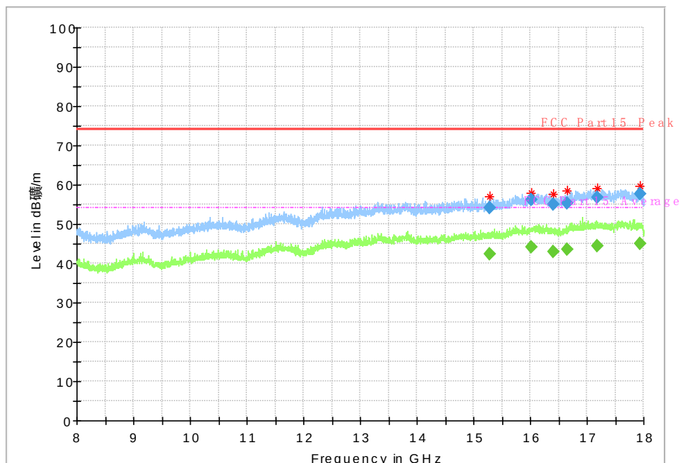
Fig. 33 Radiated Spurious Emission (802.11n-HT20, Ch165, 8 GHz-18 GHz)
