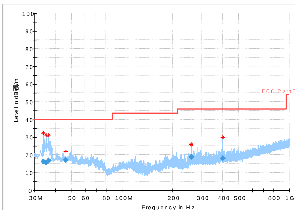
Fig. 37 Radiated Spurious Emission (802.11a, ch36, 30 MHz-1 GHz)
