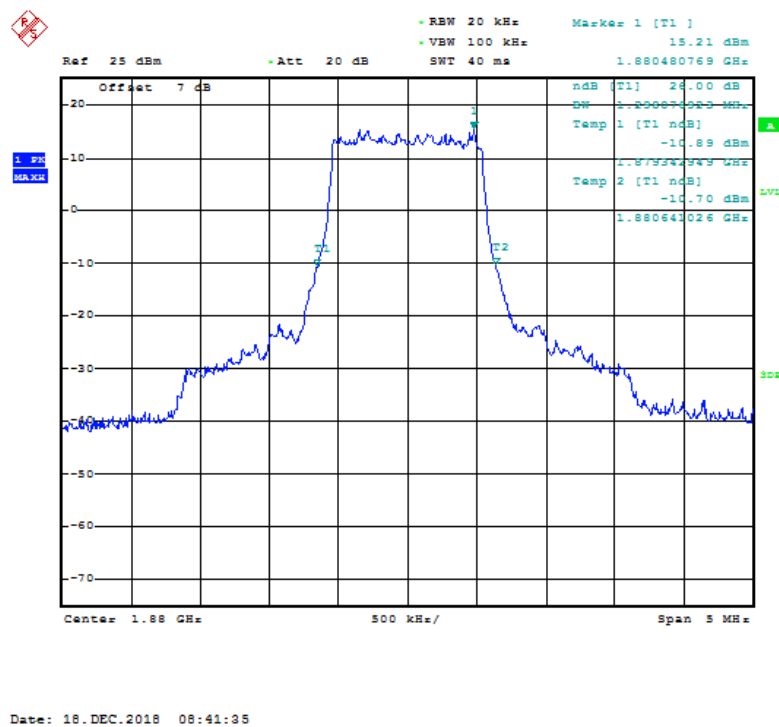
Fig.37 LTE band 2, 1.4MHz Bandwidth, QPSK (-26dBc BW)
