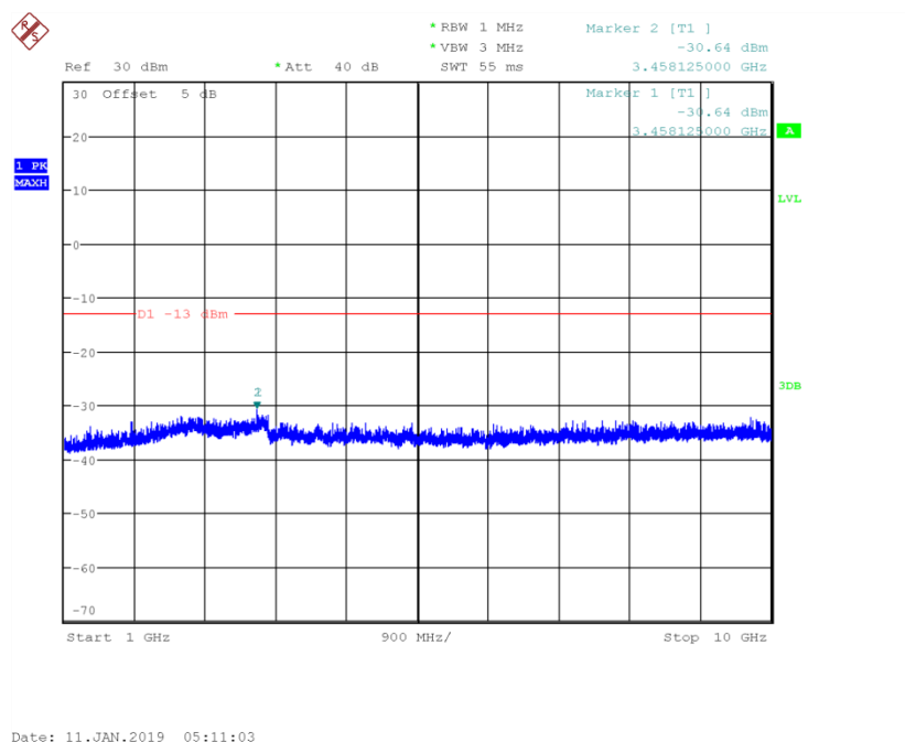
Fig.60 Channel 189: 1GHz~10GHz
