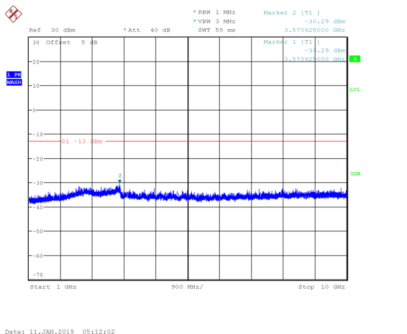
Fig.58 Channel 128: 1GHz~10GHz
