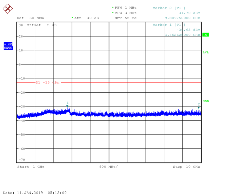
Fig.62 Channel 251: 1GHz~10GHz
