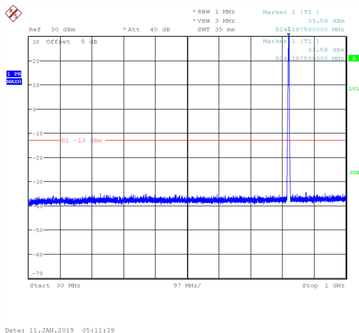
Fig.57 Channel 128: 30MHz~1GHz
