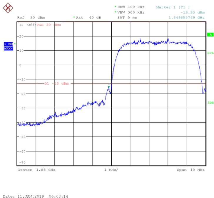
Fig.51 Channel 9262- LOW BAND EDGE BLOCK
