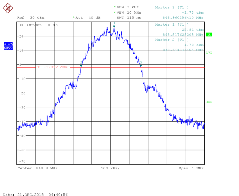
Fig.24 Channel 251- Emission Bandwidth (-26dBc BW)
