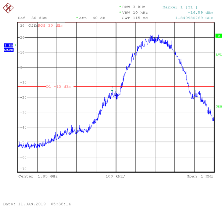
Fig.47 Channel 512- LOW BAND EDGE BLOCK
