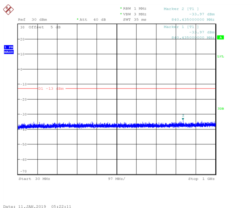
Fig.63 Channel 512: 30MHz~1GHz
