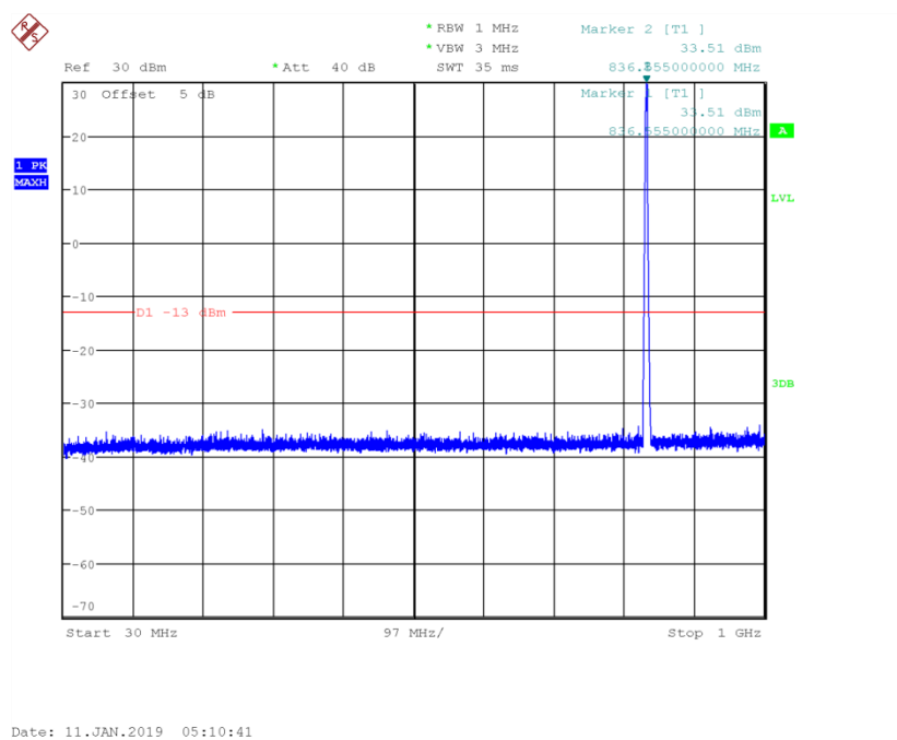
Fig.59 Channel 189: 30MHz~1GHz
