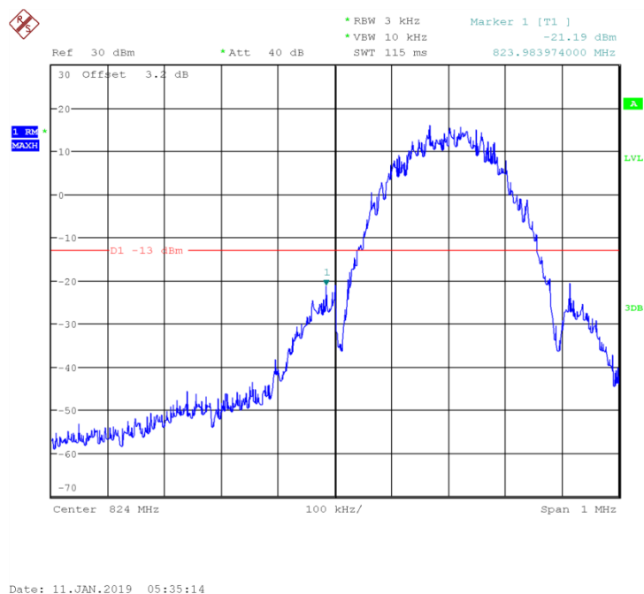
Fig.45 Channel 128- LOW BAND EDGE BLOCK
