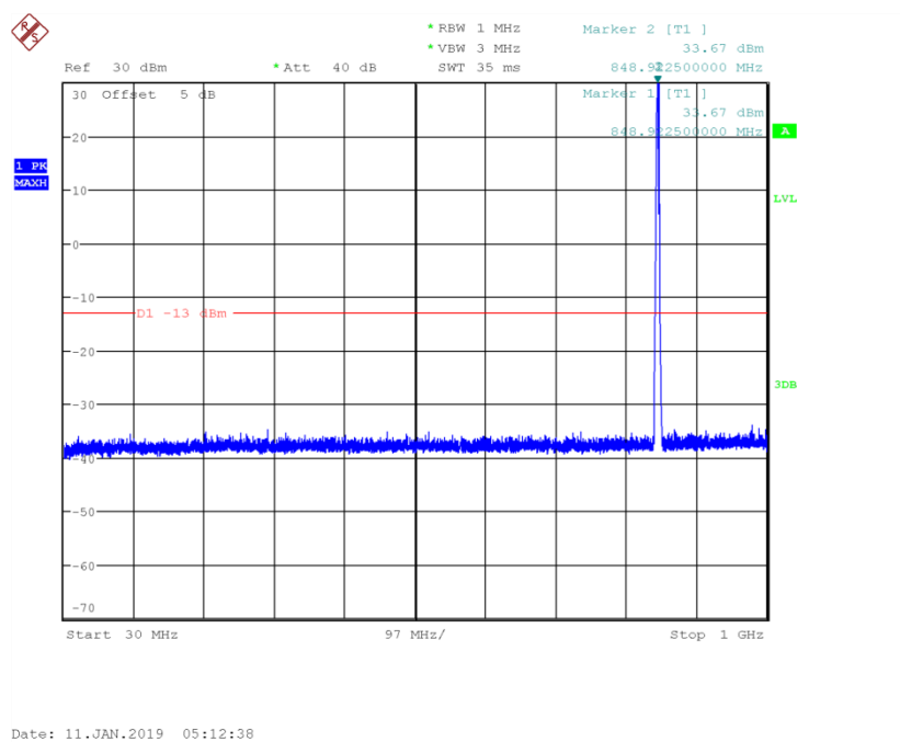
Fig.61 Channel 251: 30MHz~1GHz
