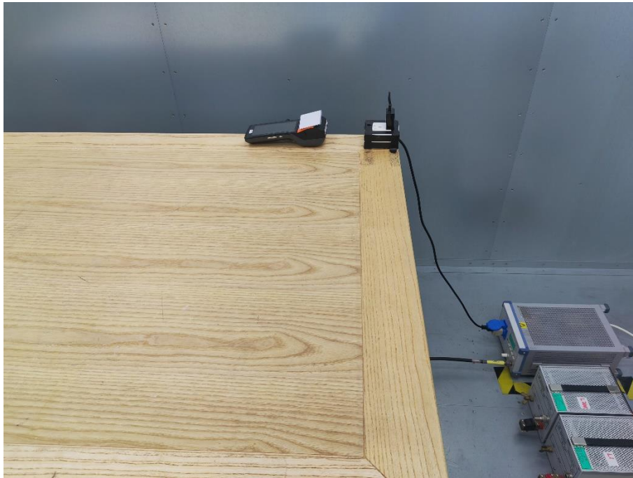
Description: Conducted Emission Test Setup
