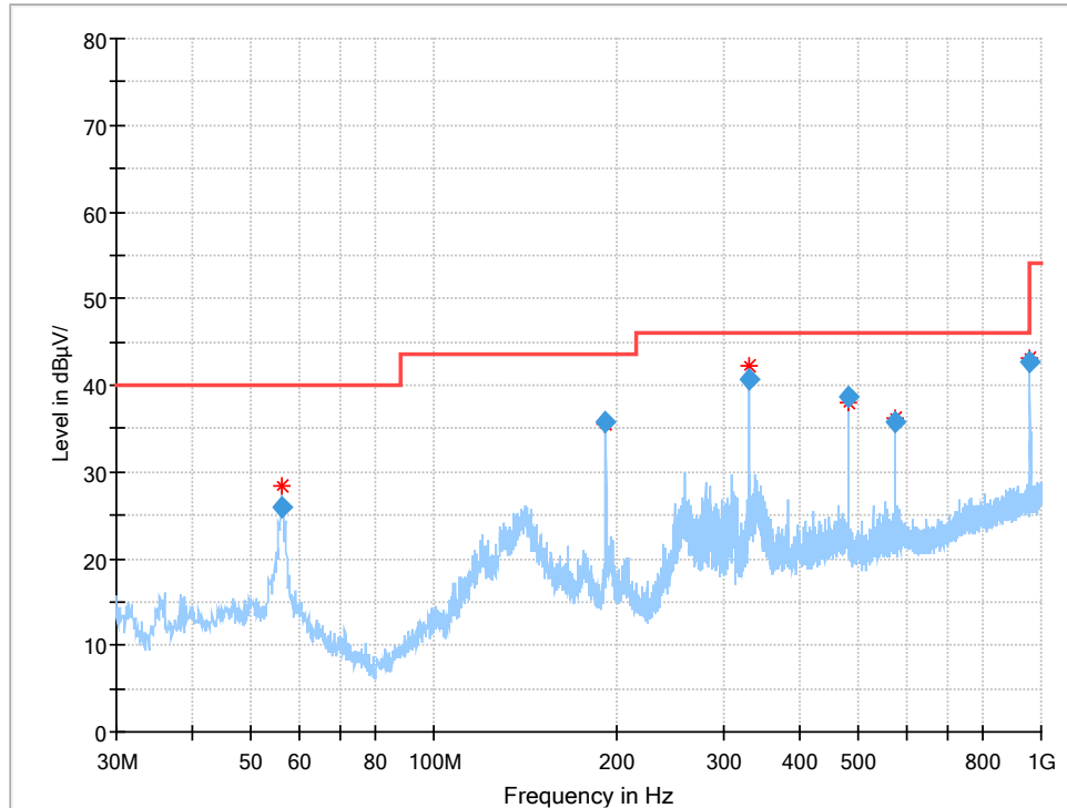
Figure A.1-1 Mode 3 (30M-1GHz)
