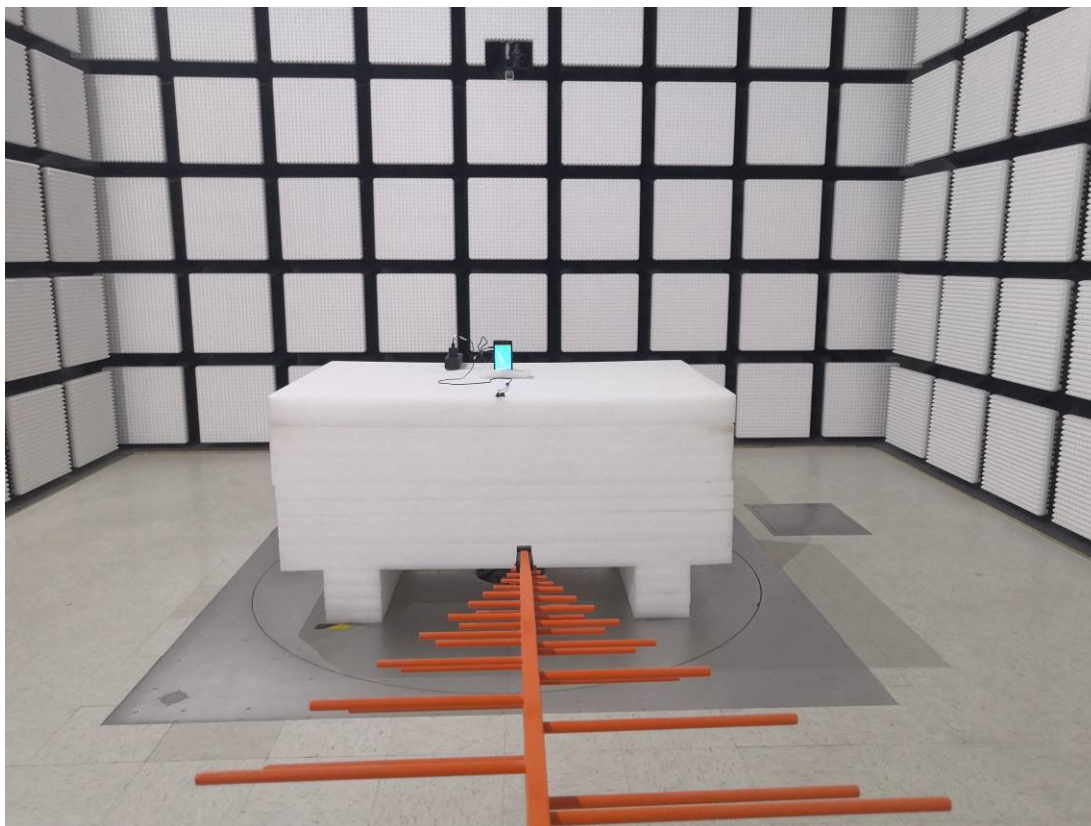
Radiated Emission Above 1GHz Type-1 View
