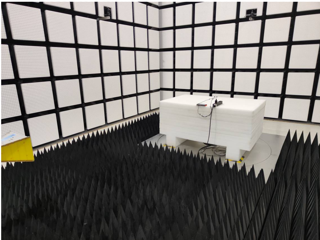
Radiated Emission Above 1G rear View Type-1 adapter 2#
