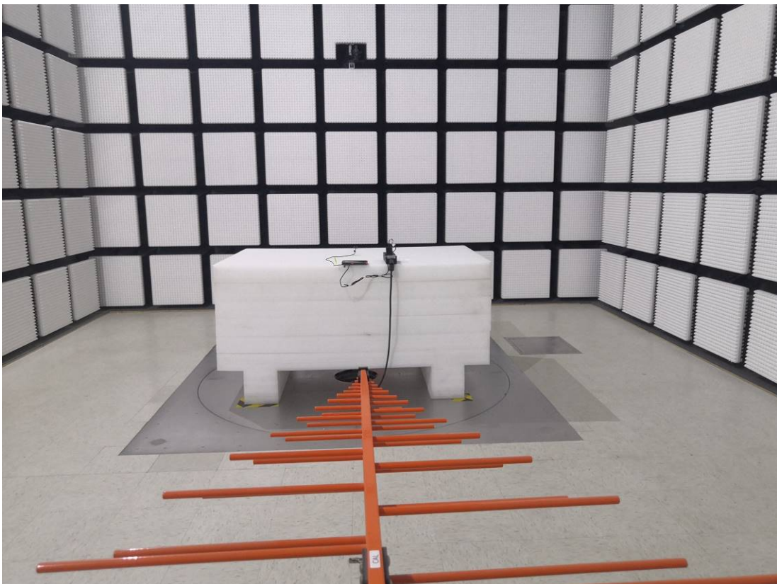
Radiated Emission Below 1G rear View Type-1 adapter 1#
