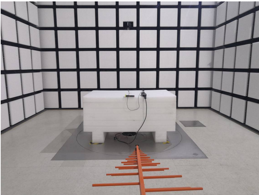
Radiated Emission Below 1G rear View Type-2 adapter 2#
