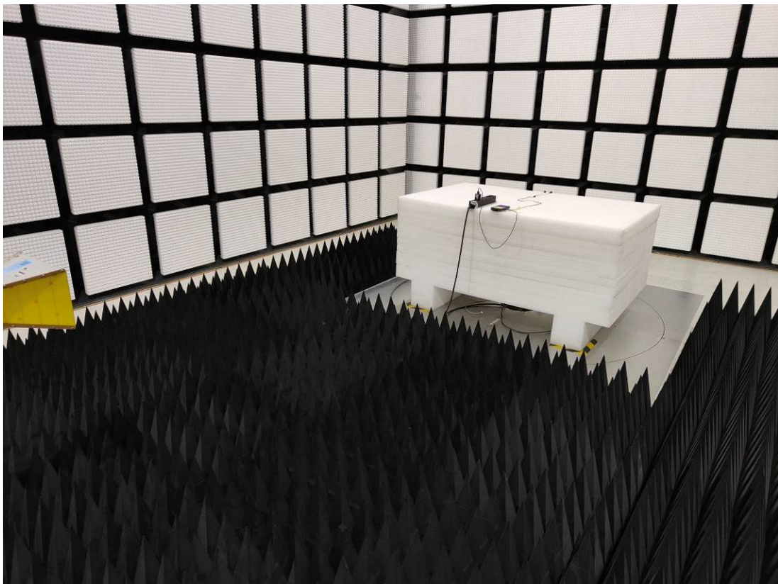
Radiated Emission Above 1G rear View Type-2 adapter 1#
