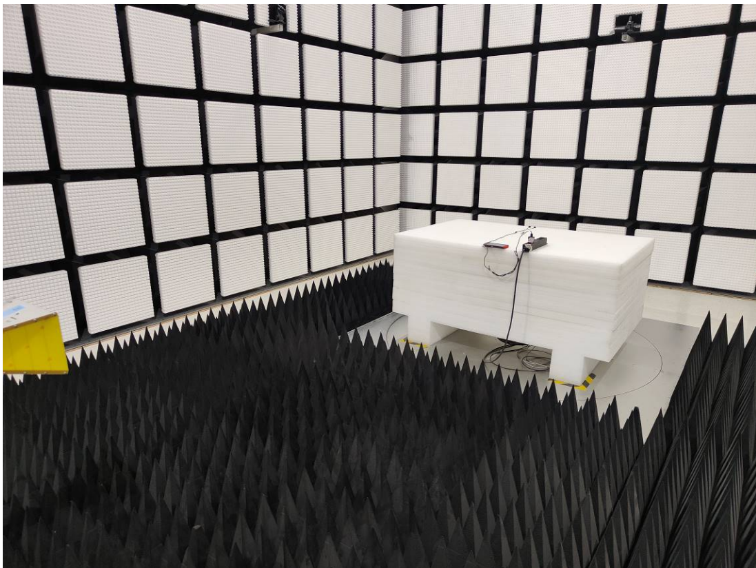
Radiated Emission Above 1G rear View Type-1 adapter 1#
