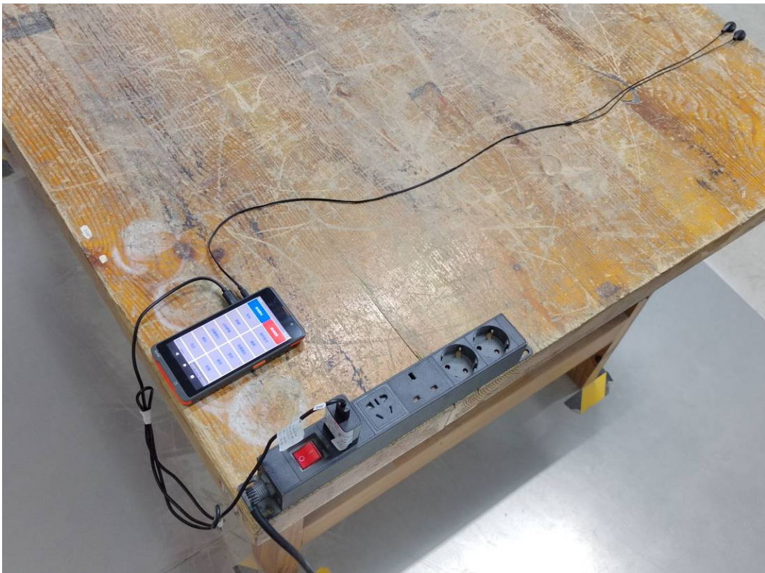
Conducted Emissions Side View Type-1 adapter 2#
