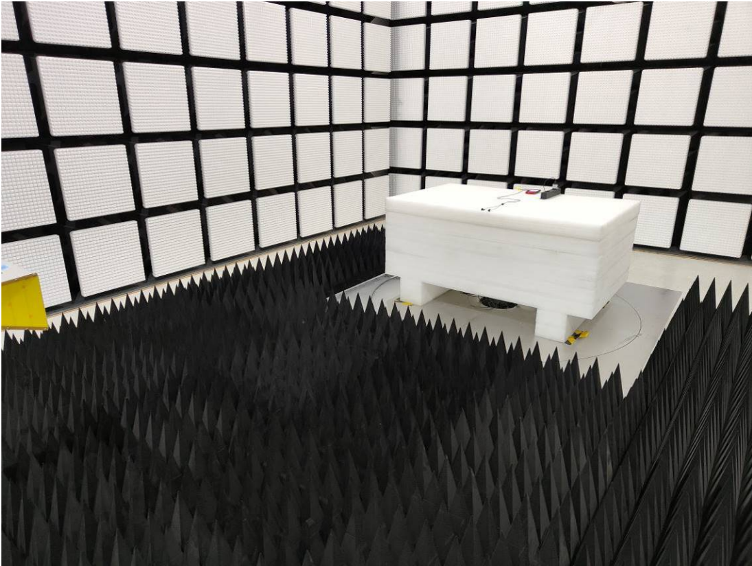
Radiated Emission Above 1G rear View Type-2 adapter 2#
