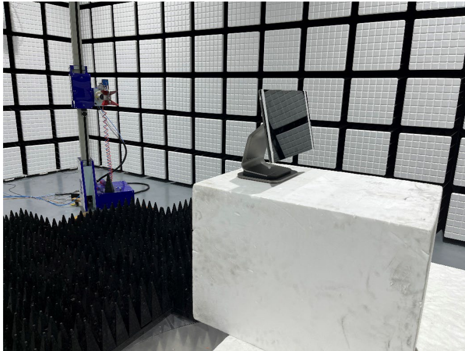
Description: Back view of Radiated Emission Test Setup (1GHz -18GHz)
