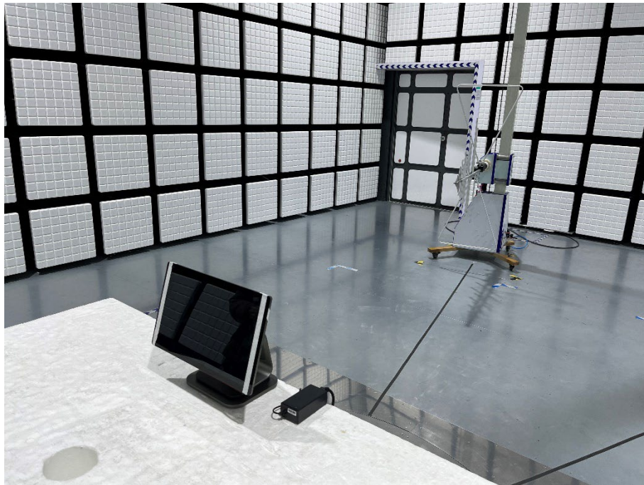
Description: Back view of Radiated Emission Test Setup (30MHz -1000MHz)
