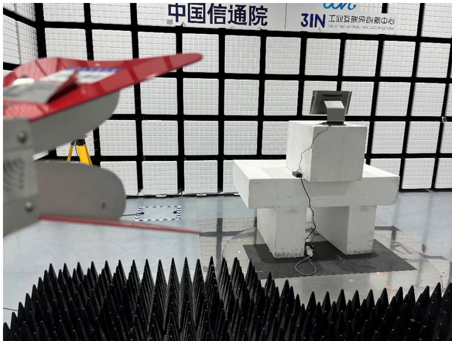
Description: Front view of Radiated Emission Test Setup (1GHz -18GHz)
