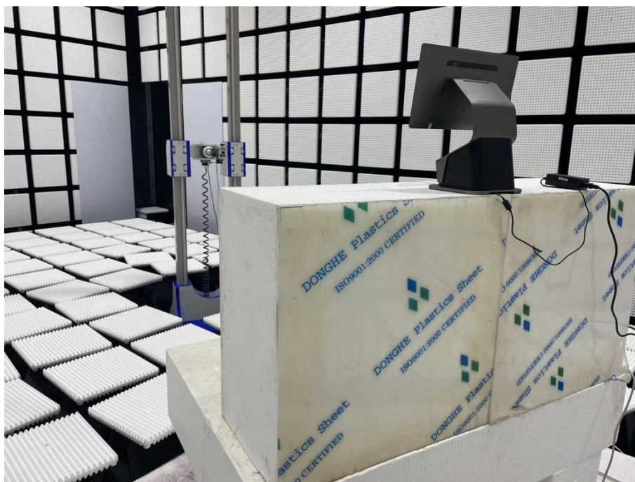
Radiated spurious Emission _26.5GHz-40GHz
