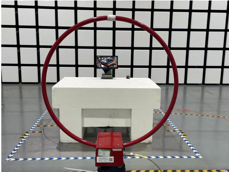
Front view of Field Radiated Emissions (Below 30MHz)
