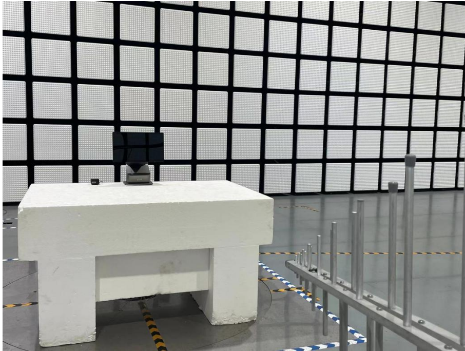
Field Radiated Emissions (Above 30MHz)
