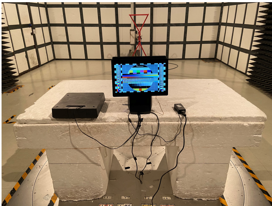
Radiated Emissions Rear Side (Below 1 GHz)
