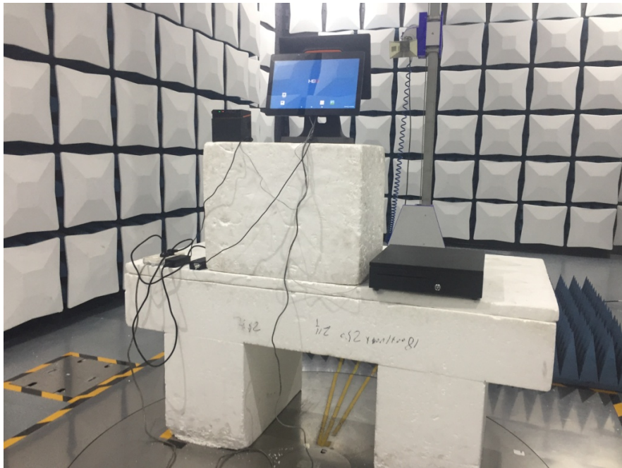
Radiated Emissions View (18GHz-40GHz)
