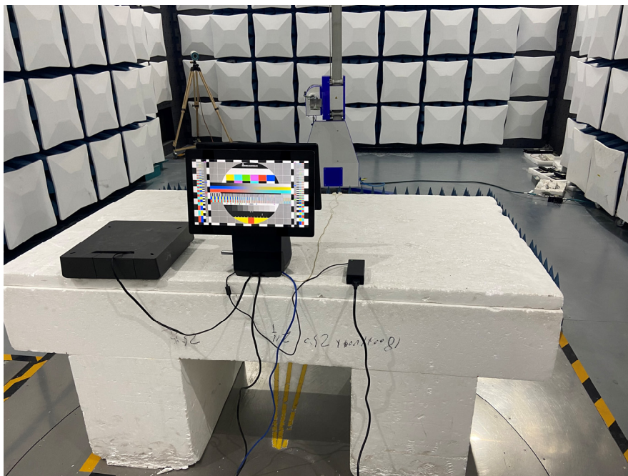
Radiated Emissions Side View (18GHz-30 GHz)
