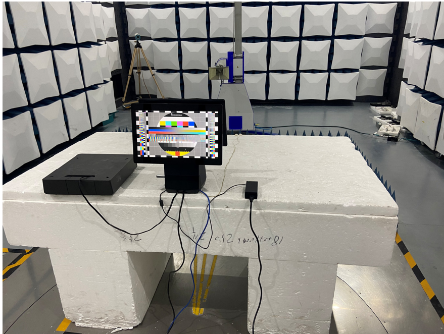
Radiated Emissions Side View (1GHz-18GHz)
