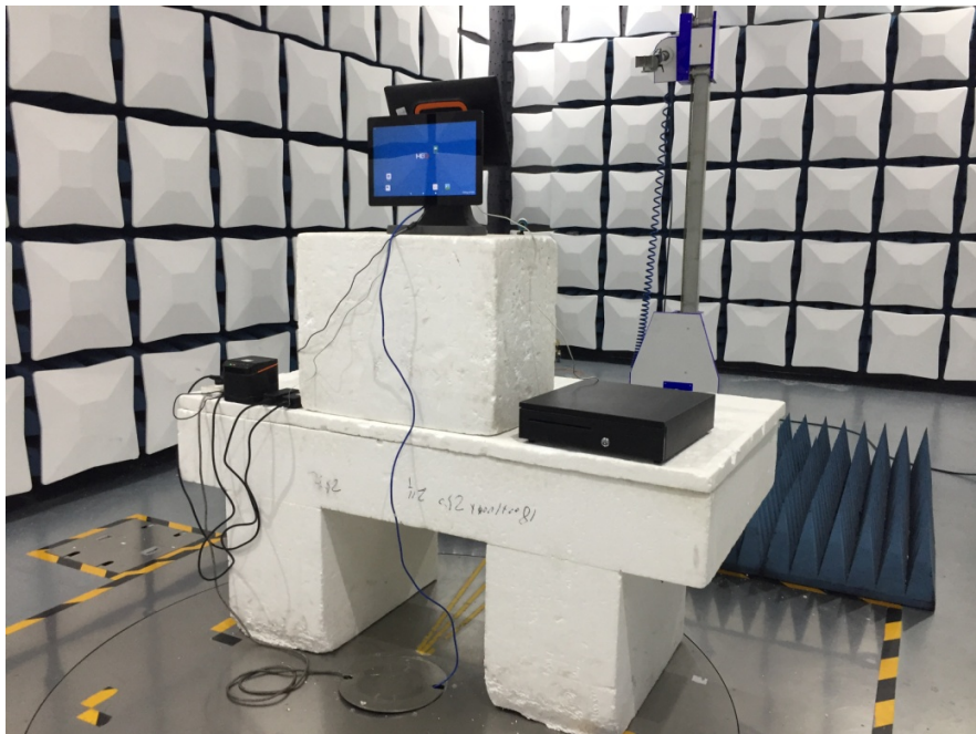
Radiated Emissions View (18GHz-25GHz)
