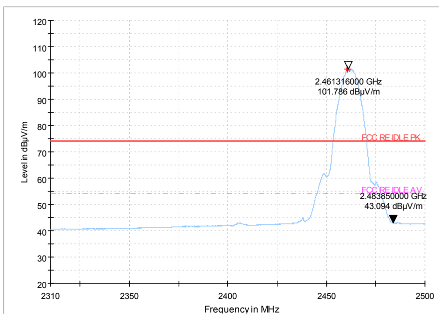
Fig 63. Radiated emission (Power): 802.11b, high channel
