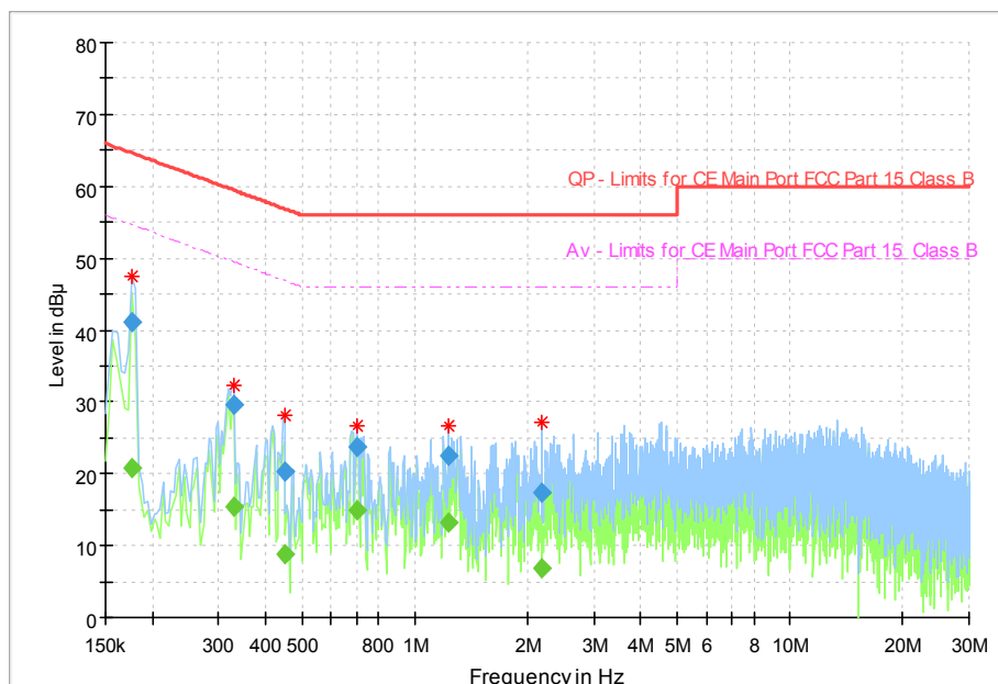
Fig 68. AC Powerline Conducted Emission
