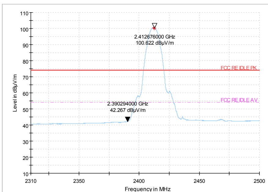
Fig 62. Radiated emission (Power): 802.11b, low channel
