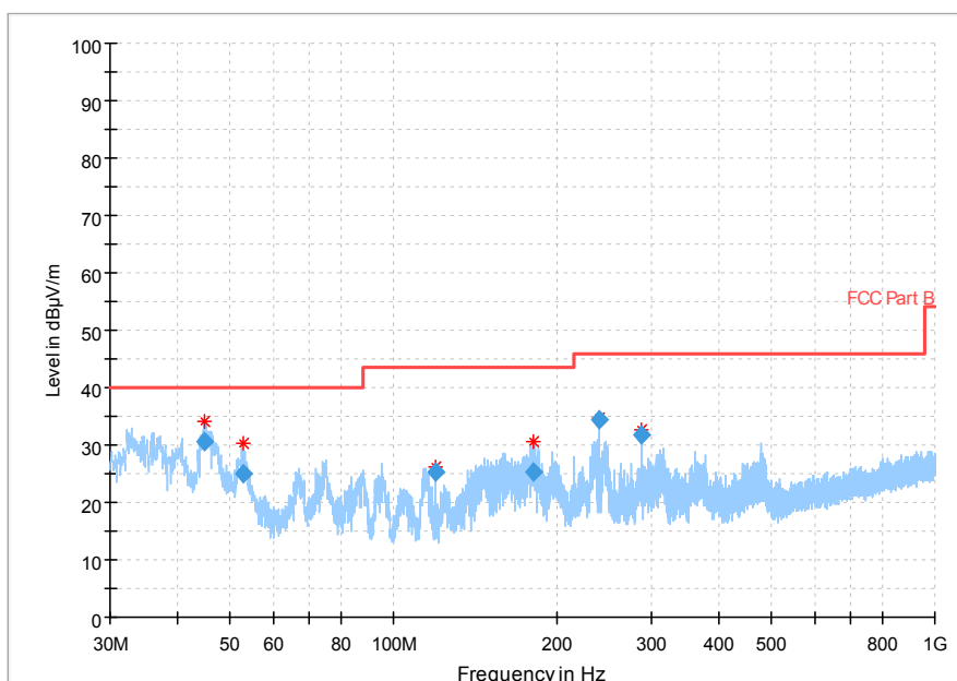
Fig 64. Radiated Spurious Emission (802.11b, Ch1,30MHz~1GHz)
