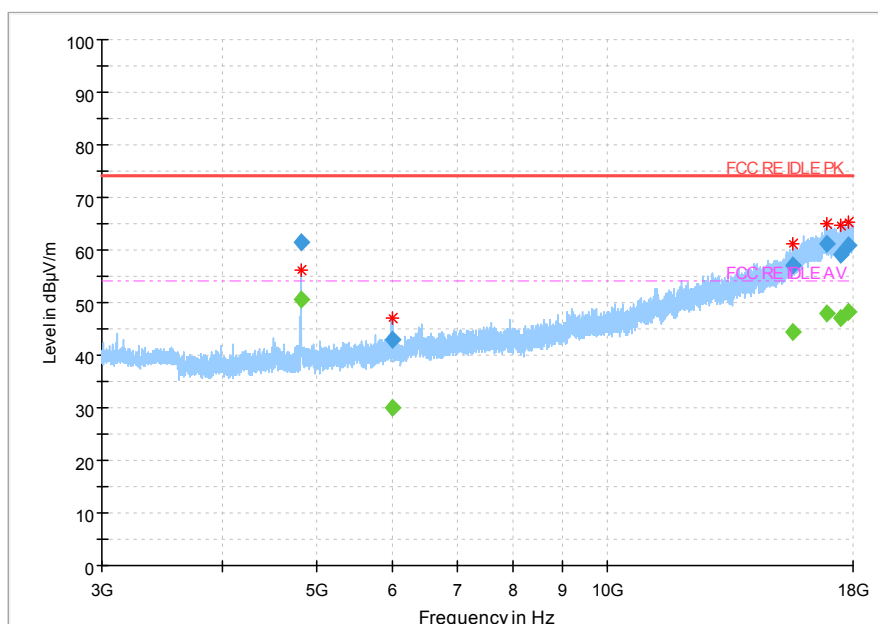
Fig 66. Radiated Spurious Emission (802.11b, Ch1, 3GHz~18GHz)
