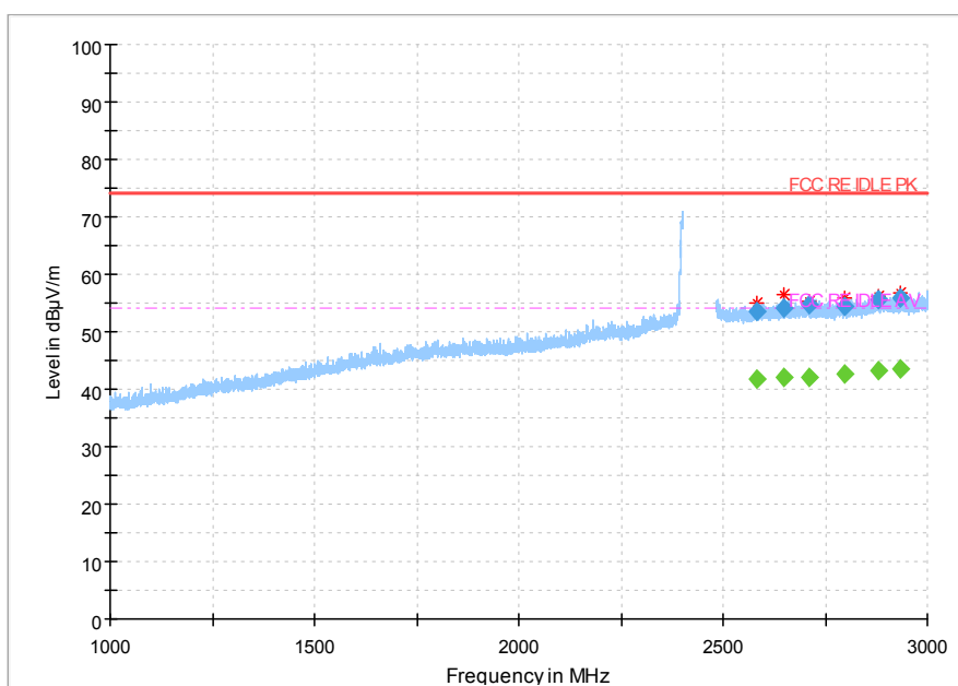
Fig 65. Radiated Spurious Emission (802.11b, Ch1,1GHz~3GHz)
