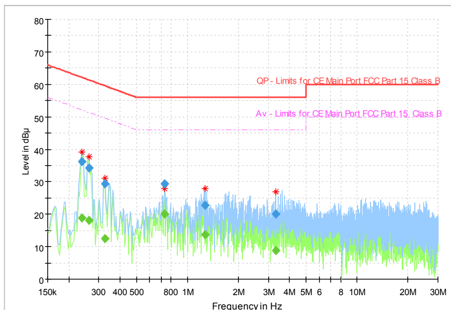
Fig 67. AC Powerline Conducted Emission
