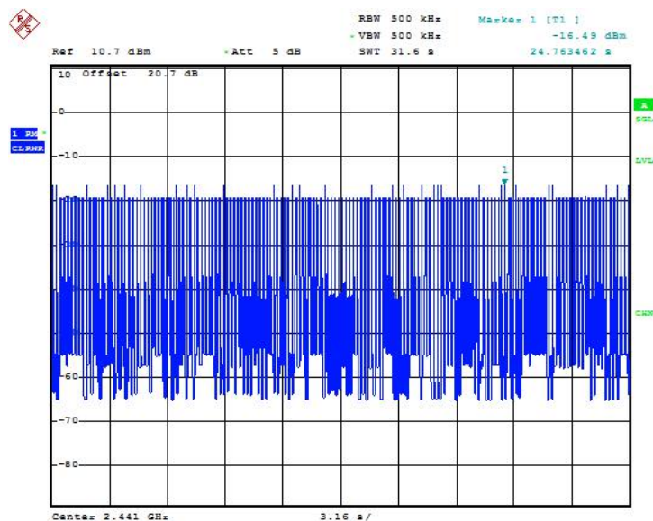
Fig.56 Time of occupancy (Dwell Time): Ch39, Packet 2-DH1
