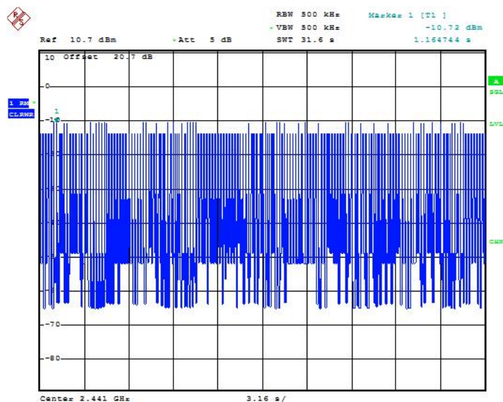
Fig.50 Time of occupancy (Dwell Time): Ch39, Packet DH1
