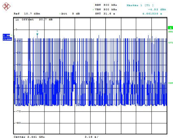
Fig.52 Time of occupancy (Dwell Time): Ch39, Packet DH3
