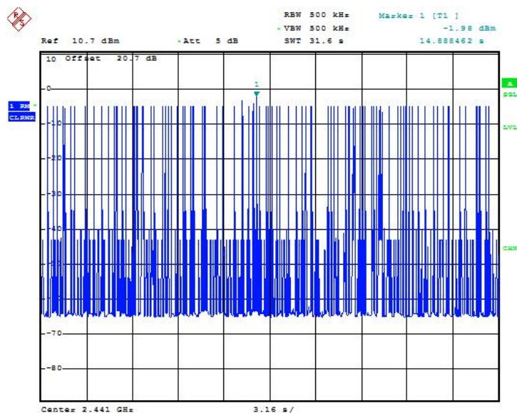
Fig.54 Time of occupancy (Dwell Time): Ch39,Packet DH5
