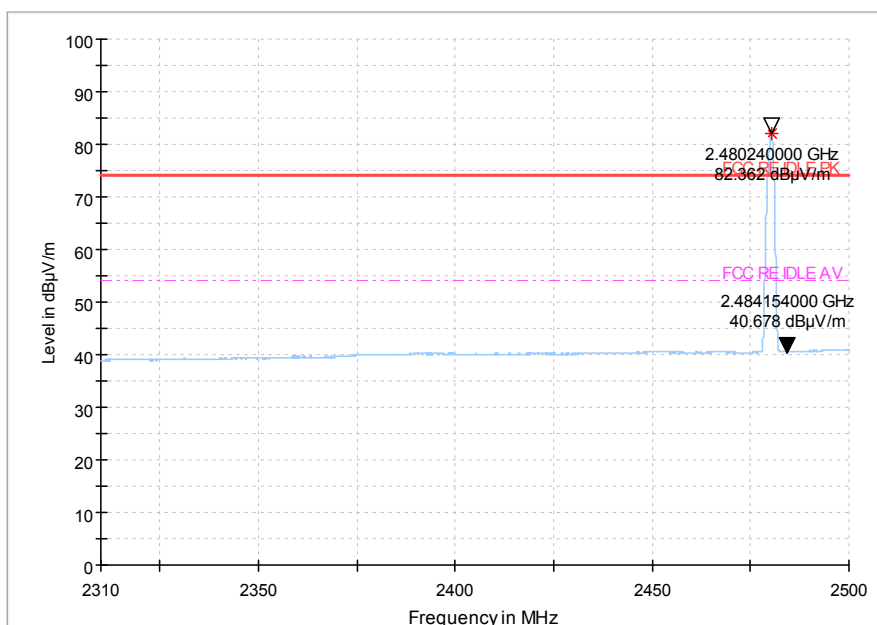
Fig.44 Radiated emission (High): \pi/4 DQPSK, high channel
