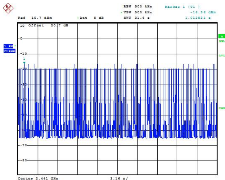
Fig.58 Time of occupancy (Dwell Time): Ch39,Packet 2-DH3
