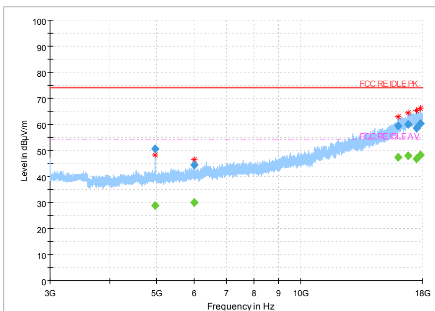
Fig.42 Radiated emission: \pi/4 DQPSK, Ch78, 3GHz~18GHz
