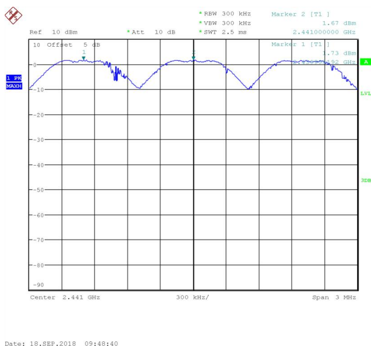
Fig.77 Carrier separation measurement: GFSK, Ch39
