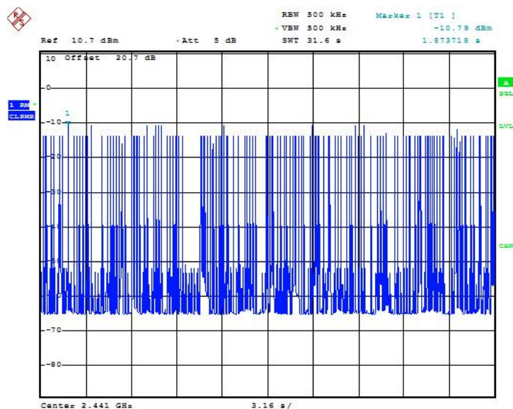
Fig.64 Time of occupancy (Dwell Time): Ch39,Packet 3-DH3
