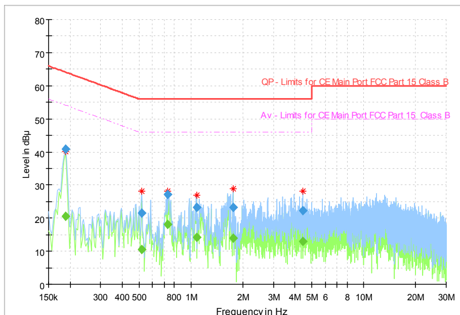
Fig.8.7 AC Powerline Conducted Emission
