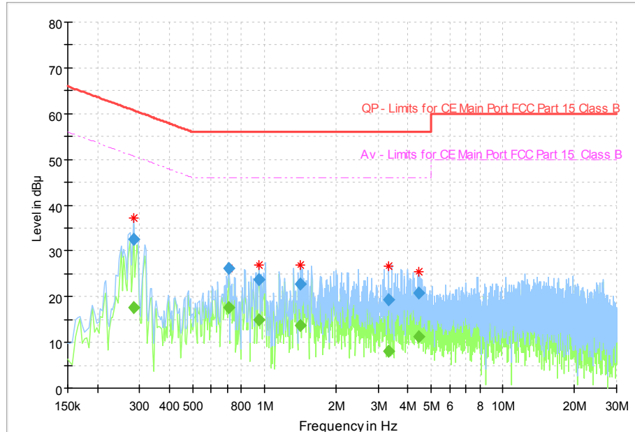
Fig.86 AC Powerline Conducted Emission
