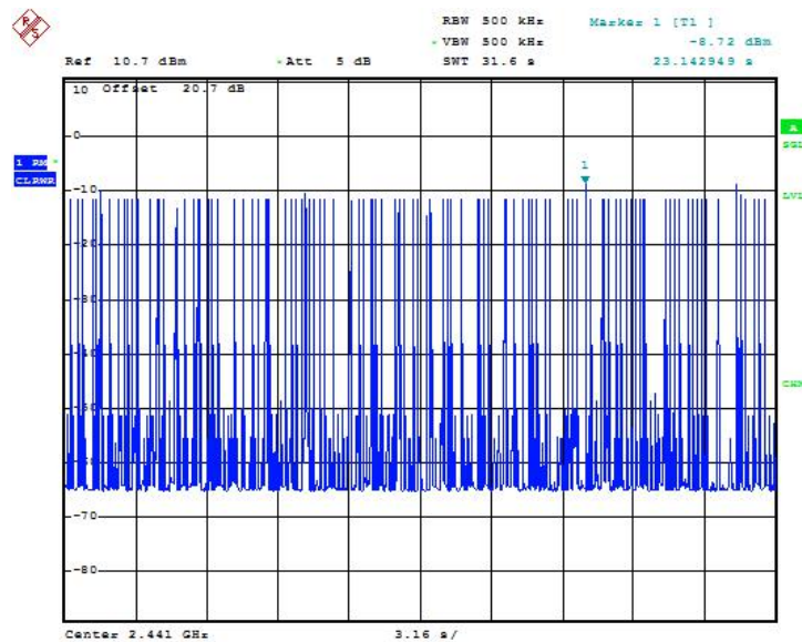
Fig.66 Time of occupancy (Dwell Time): Ch39,Packet 3-DH5
