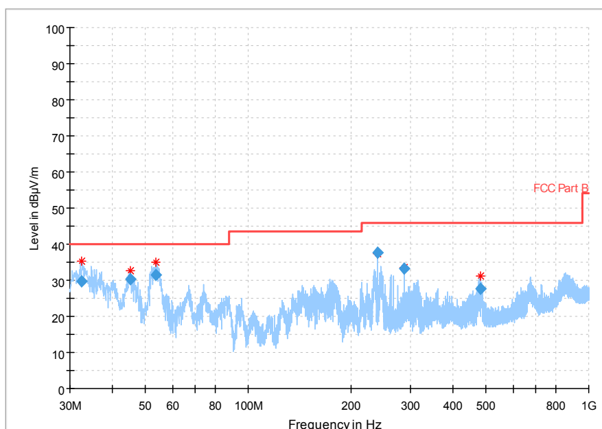
Fig.40 Radiated emission: \pi/4 DQPSK, Ch78, 30MHz~1GHz
