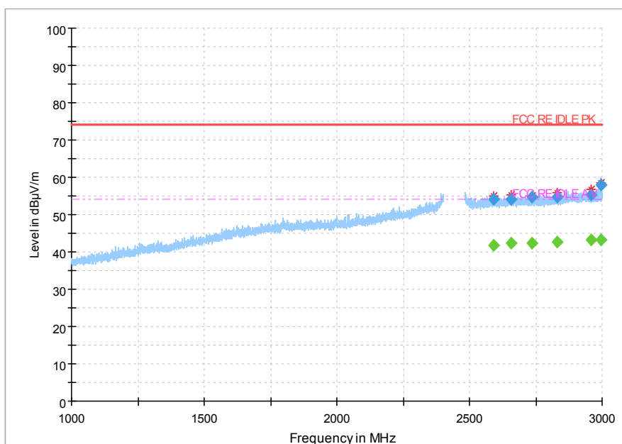
Fig.41 Radiated emission: \pi/4 DQPSK, Ch78, 1GHz~3GHz
