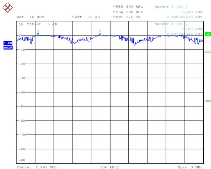
Fig.78 Carrier separation measurement: \pi/4 DQPSK, Ch39
