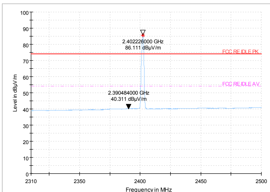
Fig.43 Radiated emission (Low): \pi/4 DQPSK, low channel
