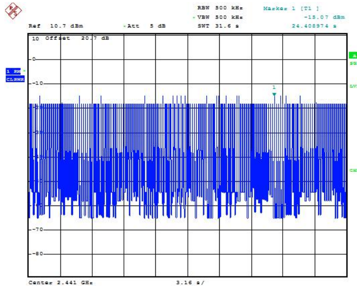
Fig.62 Time of occupancy (Dwell Time): Ch39,Packet 3-DH1
