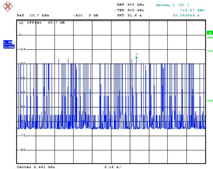
Fig.60 Time of occupancy (Dwell Time): Ch39, Packet 2-DH5
