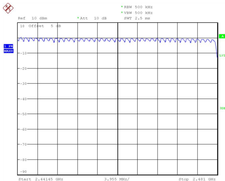
Fig.82 Number of hopping frequency: \pi/4 DQPSK, Ch0~39
