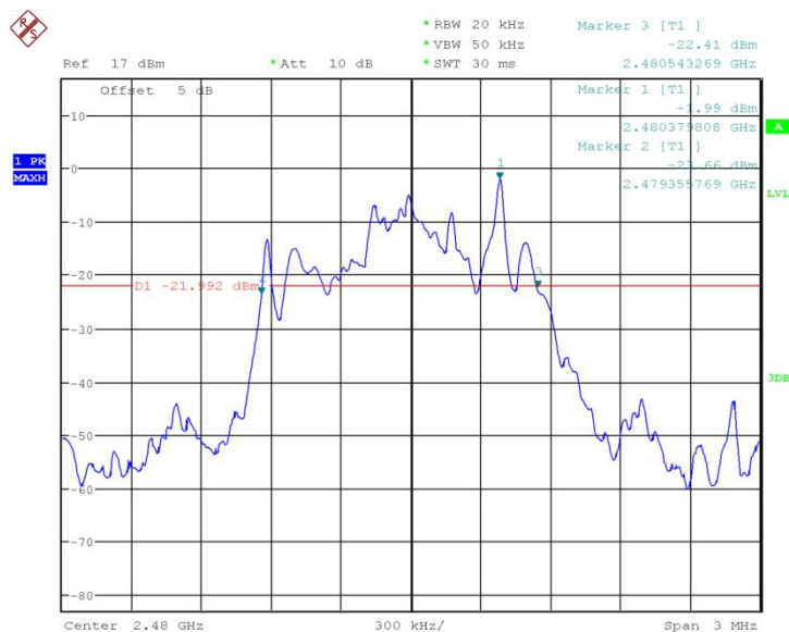
Fig.72 20dB Bandwidth: \pi/4 DQPSK, Ch39
