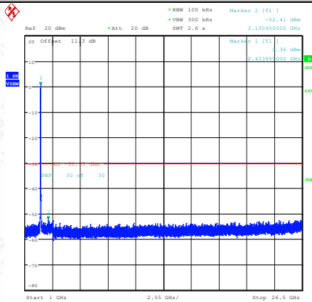
11N40SISO-Ant1-2437-1000~26500-PASS
