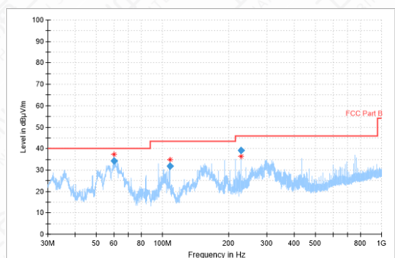
RSE-11N(40M)-CH9-30MHz-1GHz
