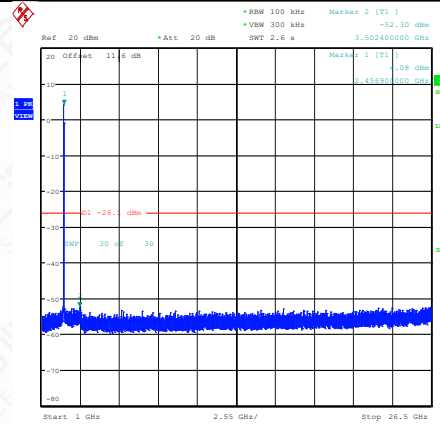
11G-Ant1-2462-1000~26500-PASS
