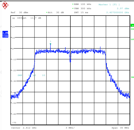
11N20SISO-Ant1-2412-0~Reference-PASS
