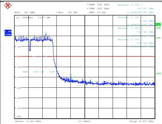
11N40SISO-Ant1-2452-PASS
