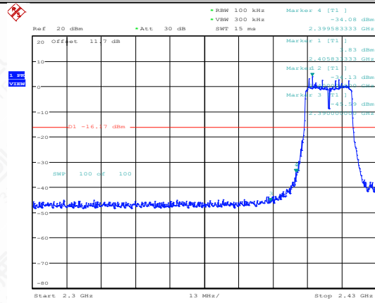
11N20SISO-Ant1-2412-PASS
