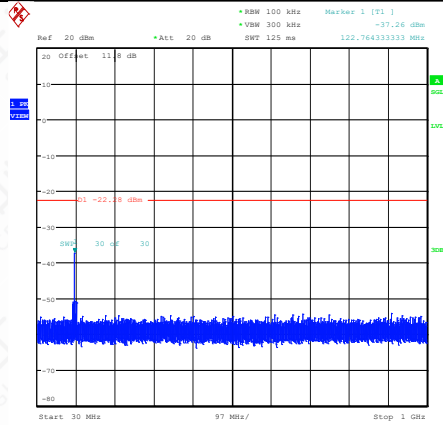
11B-Ant1-2437-30~1000-PASS
