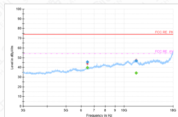
RSE-11N(40M)-CH3-3GHz-18GHz
