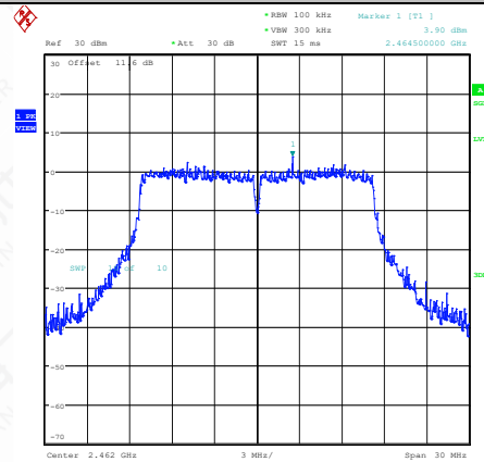
11G-Ant1-2462-0~Reference-PASS
