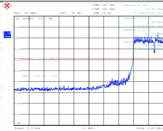
11N40SISO-Ant1-2422-PASS
