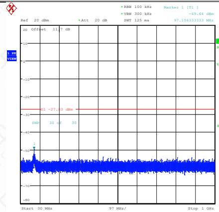
11N20SISO-Ant1-2412-30~1000-PASS
