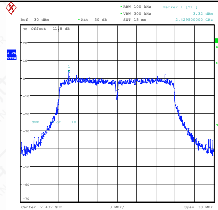
11N20SISO-Ant1-2437-0~Reference-PASS
