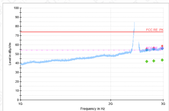
RSE-11N(40M)-CH3-1GHz-3GHz
