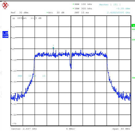
11N40SISO-Ant1-2437-0~Reference-PASS
