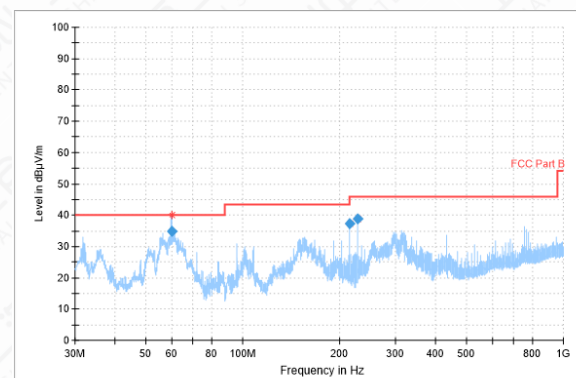
RSE-11N(40M)-CH3-30MHz-1GHz
