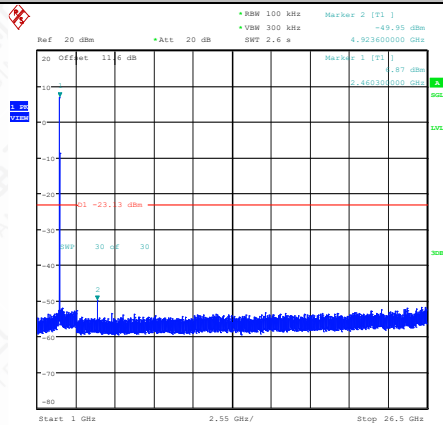
11B-Ant1-2462-1000~26500-PASS
