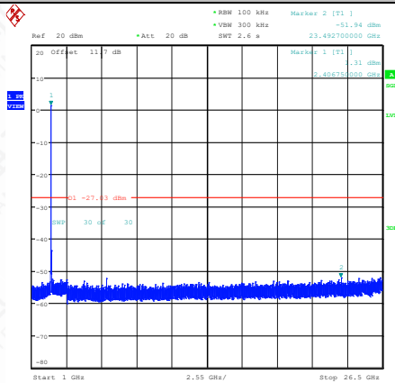
11N20SISO-Ant1-2412-1000~26500-PASS
