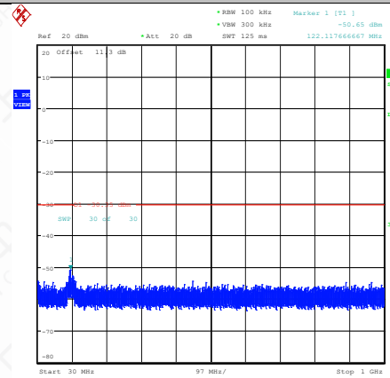
11N40SISO-Ant1-2437-30~1000-PASS
