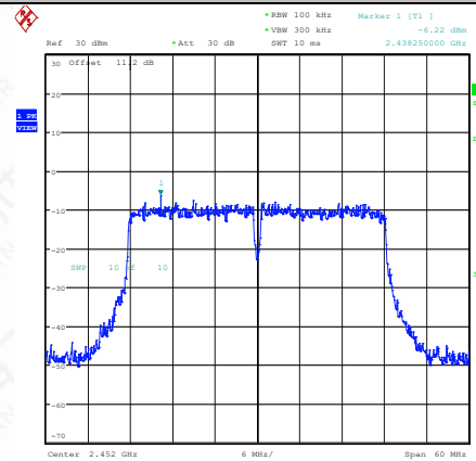
11N40SISO-Ant1-2452-0~Reference-PASS
