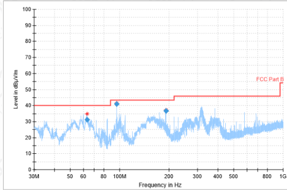
RSE-11B-CH1-30MHz-1GHz
