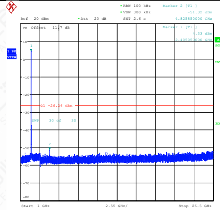
11G-Ant1-2412-1000~26500-PASS
