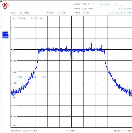
11G-Ant1-2437-0~Reference-PASS
