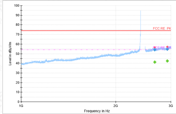
RSE-11B-CH1-1GHz-3GHz
