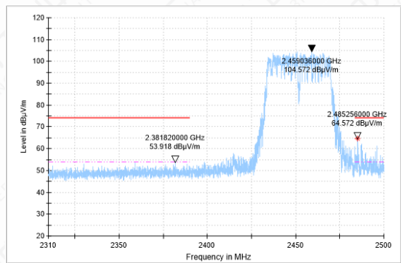
Bandedeg-11N(40M)-CH9-PK-38
