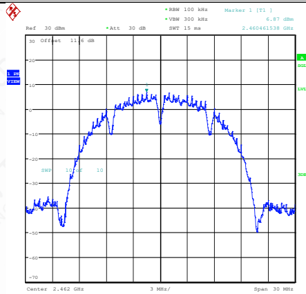
11B-Ant1-2462-0~Reference-PASS
