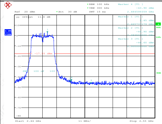
11N20SISO-Ant1-2462-PASS
