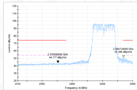
Bandedeg-11N(40M)-CH9-AV-38-2.71
