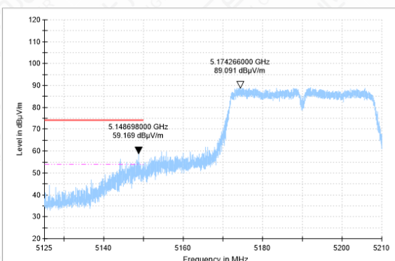
Bandedge-11AC(40M)-CH38-PK
