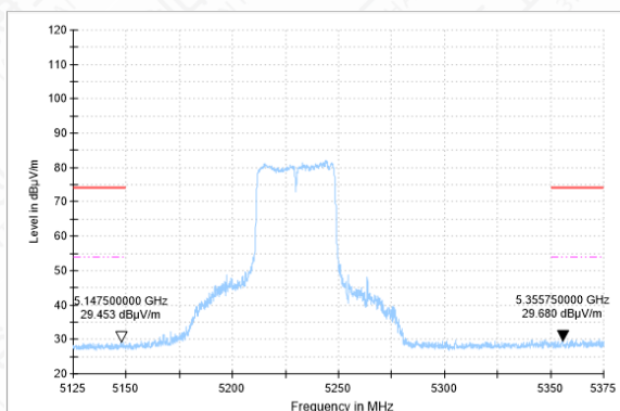
Bandedge-11AC(40M)-CH46-AV
