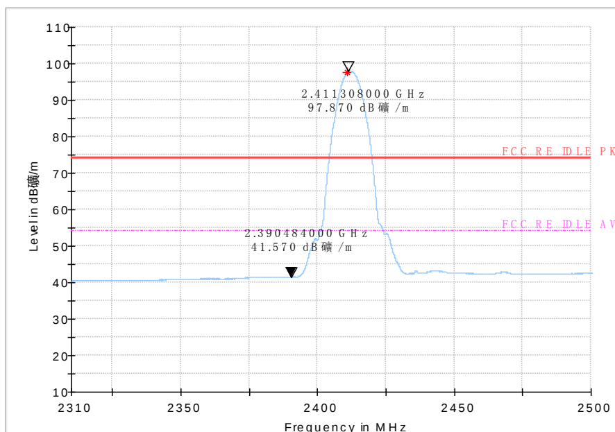
Fig 82. Radiated emission (Power): 802.11b, low channel
