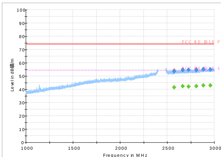
Fig 85. Radiated Spurious Emission (802.11b,Ch11,1GHz~3GHz)
