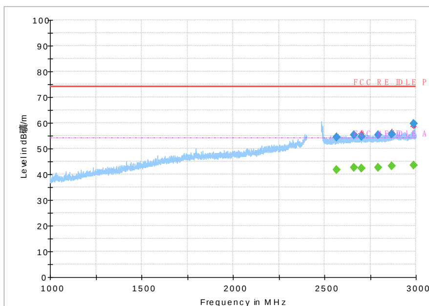
Fig 80. Radiated Spurious Emission (802.11b,Ch11,1GHz~3GHz)
