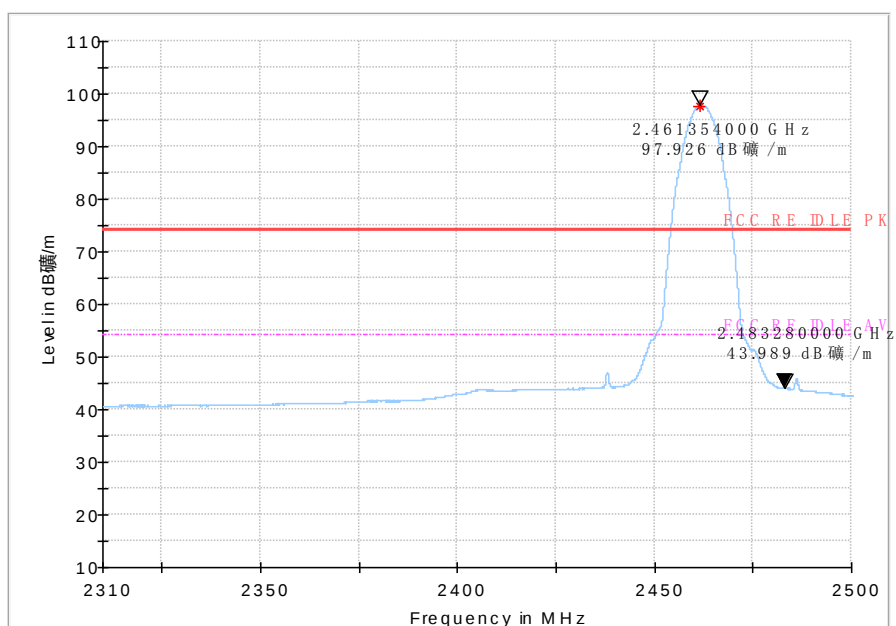
Fig 78. Radiated emission (Power): 802.11b, high channel
