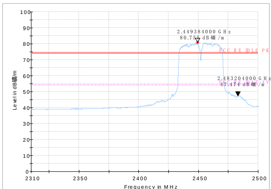
Fig 73. Radiated emission (Power): 802.11 n-40MHz, high channel
