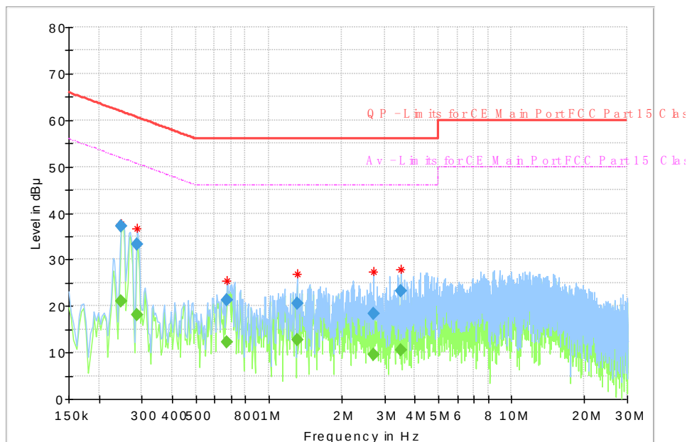
Fig 87. AC Powerline Conducted Emission
