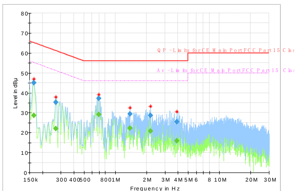
Fig 89. AC Powerline Conducted Emission
