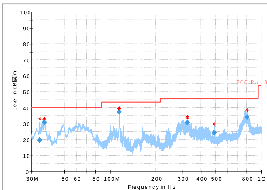
Fig 84. Radiated Spurious Emission (802.11b,Ch11,30MHz~1GHz)
