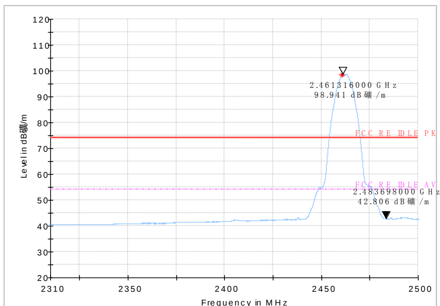
Fig 83. Radiated emission (Power): 802.11b, high channel
