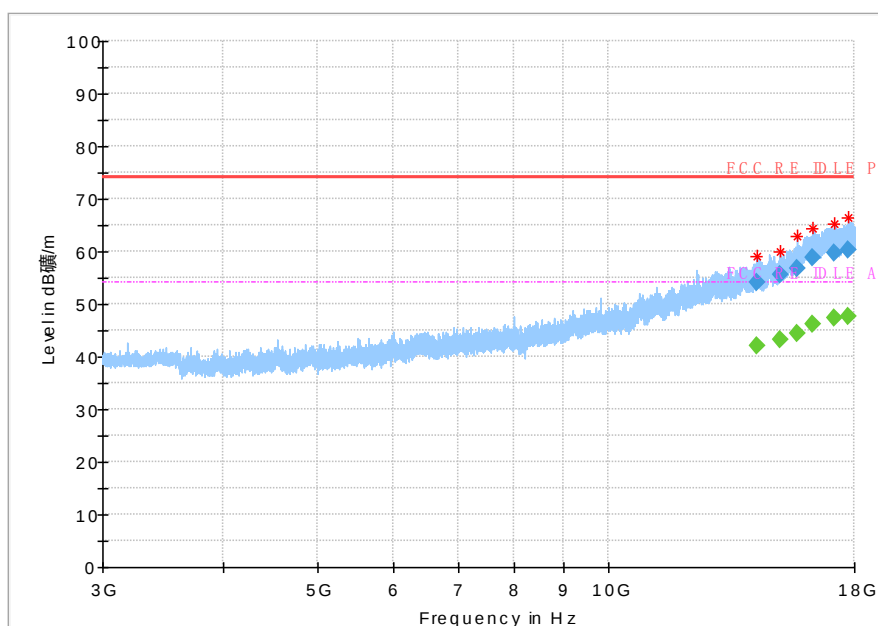
Fig 86. Radiated Spurious Emission (802.11b,Ch11,3GHz~18GHz)
