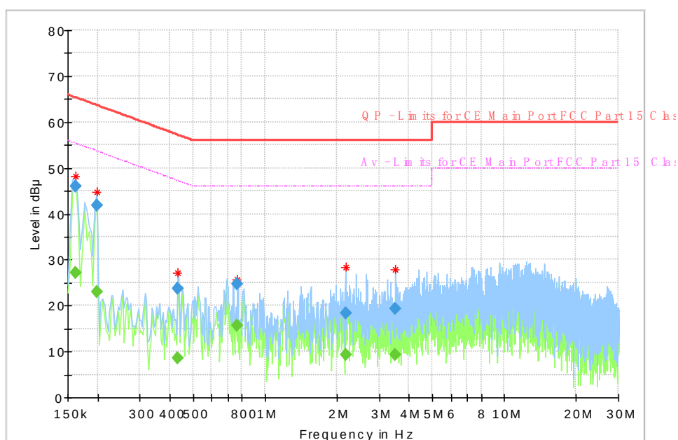
Fig 88. AC Powerline Conducted Emission
