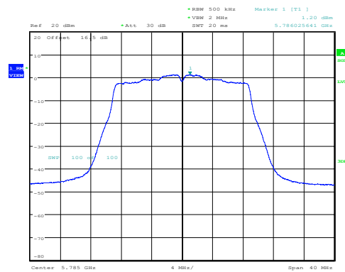
11AC20SISO-Ant1-5785-PASS
