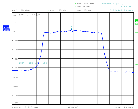
11AX20SISO-Ant1-5825-PASS
