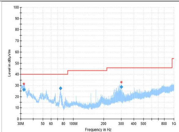
RSE-11AC-CH157-30MHz-1GHz
