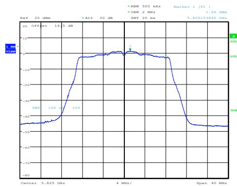
11AC20SISO-Ant1-5825-PASS
