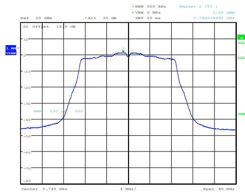
11AC20SISO-Ant1-5745-PASS
