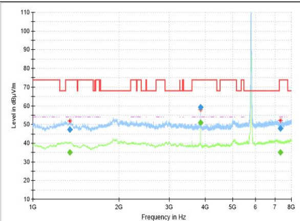
RSE-11AC-CH157-1GHz-8GHz
