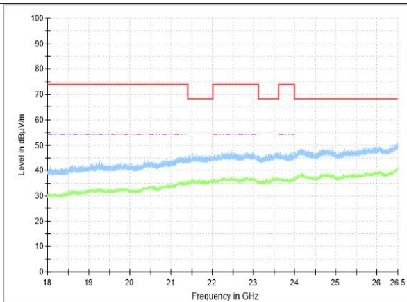
RSE-11N-CH165-18G-26.5G
