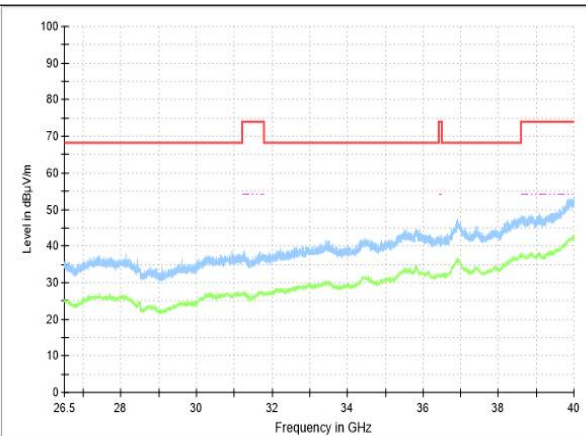
RSE-11N-CH165-26.5G-40G
