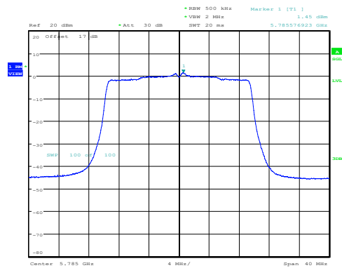
11AX20SISO-Ant1-5785-PASS
