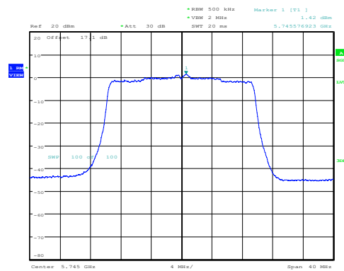
11AX20SISO-Ant1-5745-PASS
