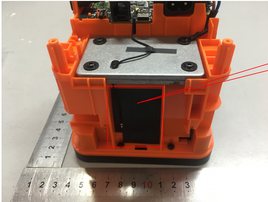
GPRS Antenna
