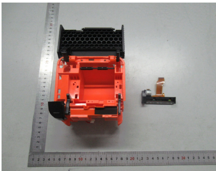
EUT –Cover off View-6
