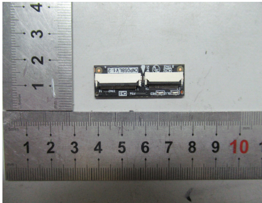
EUT –PCB 2 Top View
