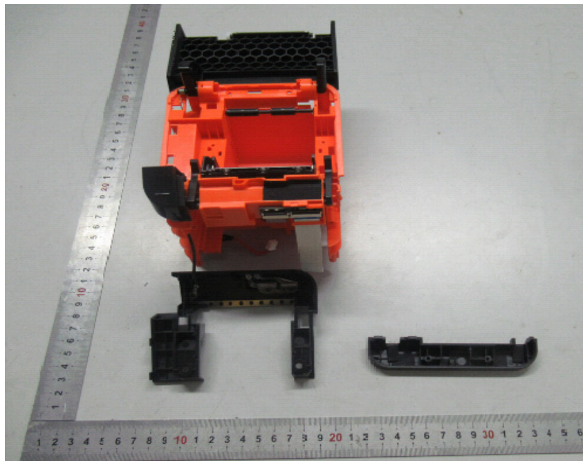
EUT –Cover off View-4
