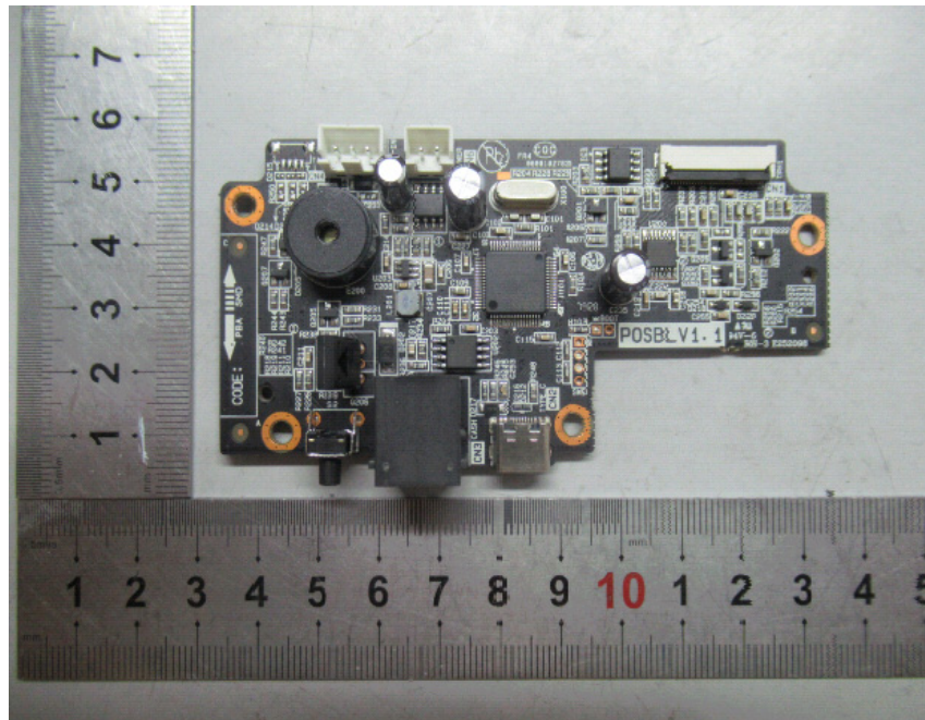
EUT –PCB 1 Bottom View
