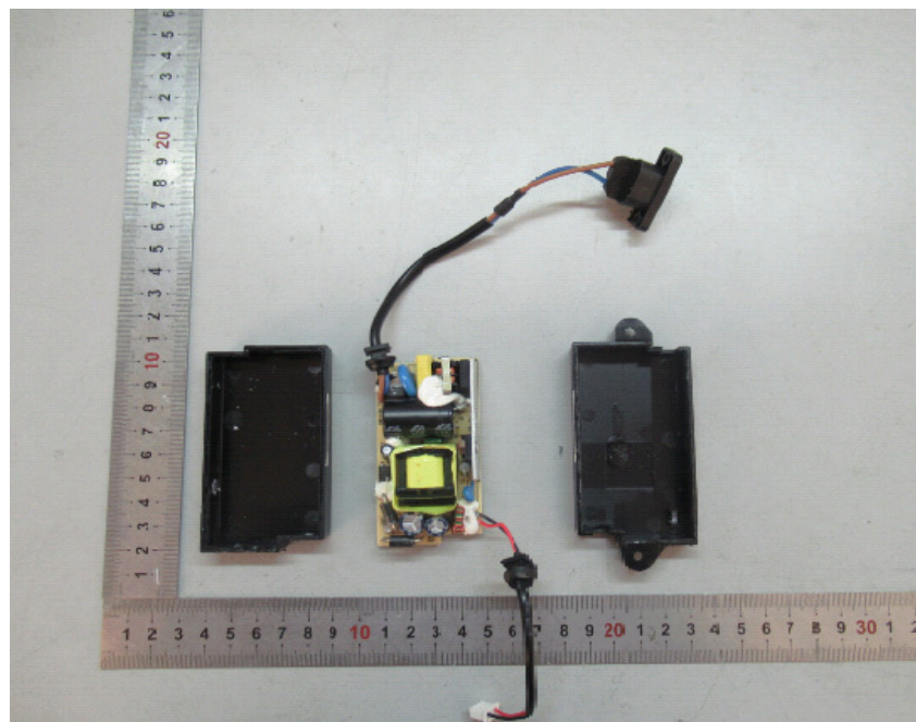
EUT – Adapter Cover off View 1
