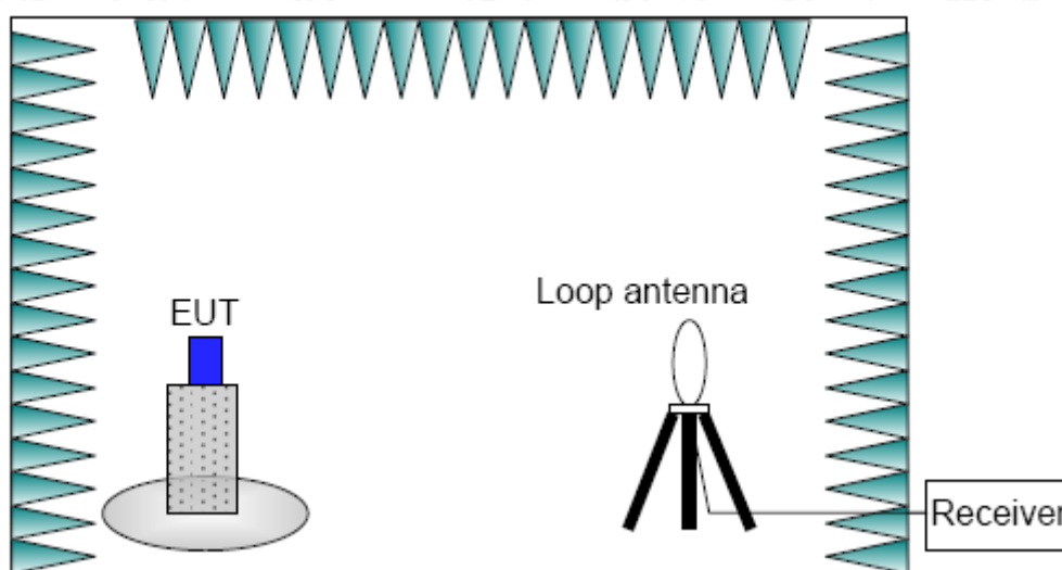
Figure 6.3.2.2-1 Electric Field Radiated Emissions (Below 30MHz) Connection Diagram
