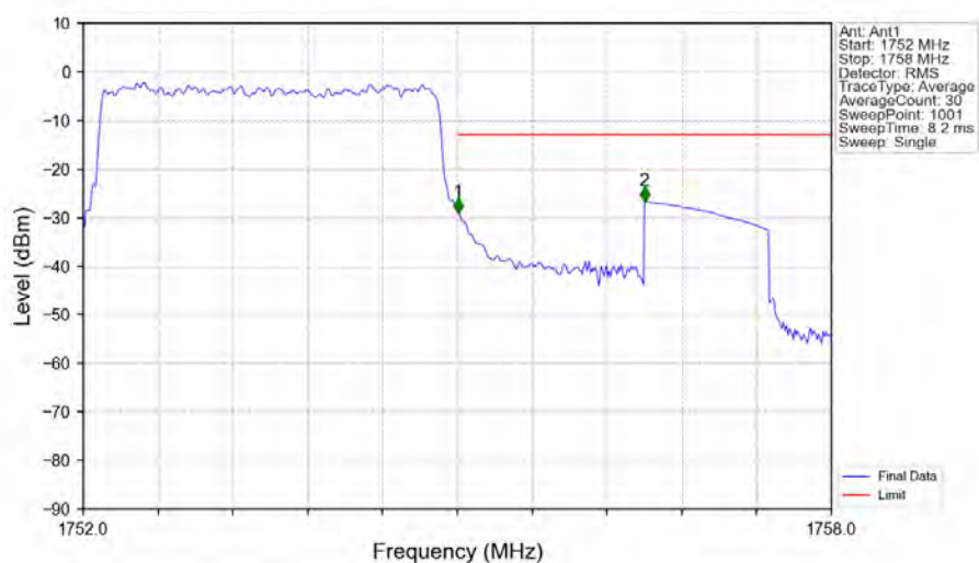
Band4_3MHz_QPSK_HCH_1753.5MHz_RB 15_0_NTNV
