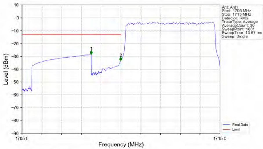
Band4_5MHz_QPSK_LCH_1712.5MHz_RB_25_0_NTNV
