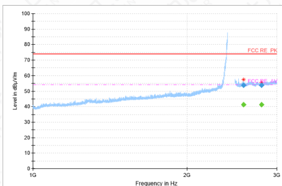
RSE-11G-CH1-1GHz-3GHz
