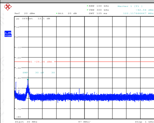
11N40MIMO-Ant2-2437-30~1000-PASS
