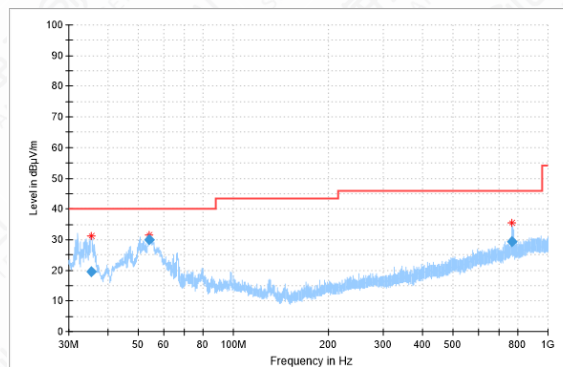
RSE-11G-CH1-30MHz-1GHz
