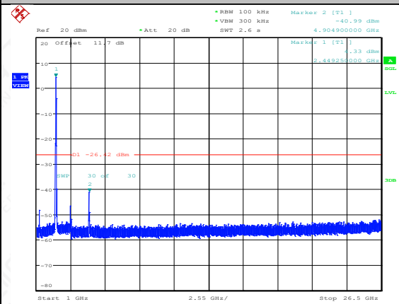
11N40MIMO-Ant1-2452-1000~26500-PASS
