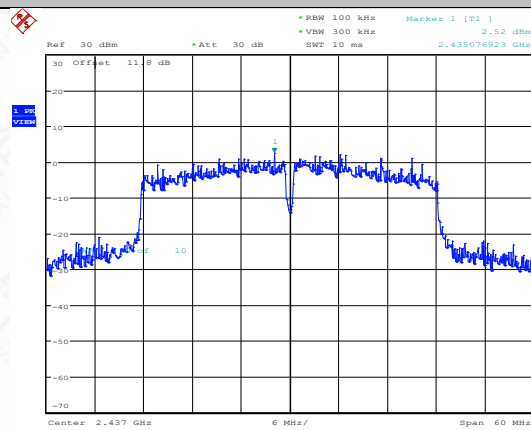
11N40MIMO-Ant1-2437-0~Reference-PASS
