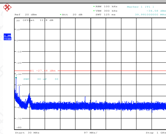
11N40MIMO-Ant1-2437-30~1000-PASS
