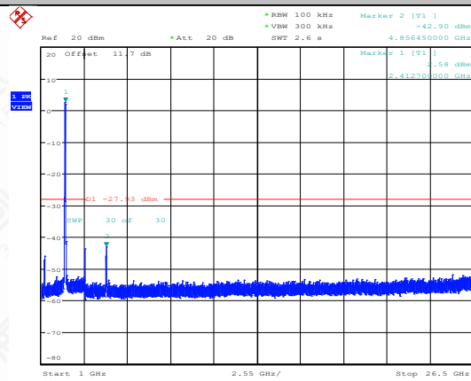
11N40MIMO-Ant1-2422-1000~26500-PASS
