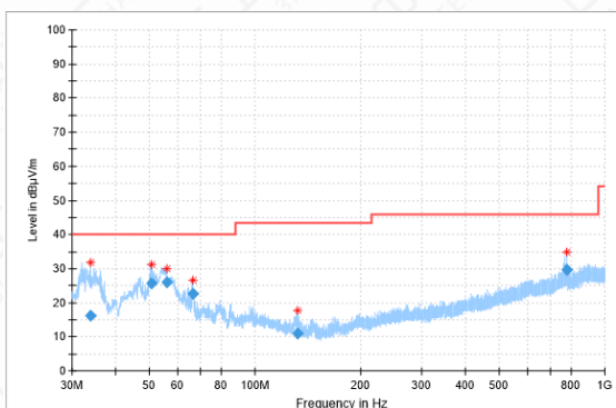
RSE-11G-CH6-30MHz-1GHz
