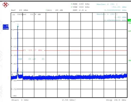
11N40MIMO-Ant2-2452-1000~26500-PASS
