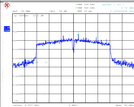
11N40MIMO-Ant2-2437-0~Reference-PASS
