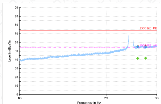
RSE-11G-CH6-1GHz-3GHz
