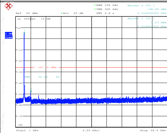
11N40MIMO-Ant2-2422-1000~26500-PASS
