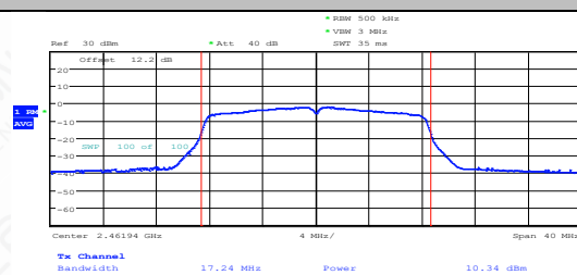
11G-CDD-Ant1-2462-PASS
