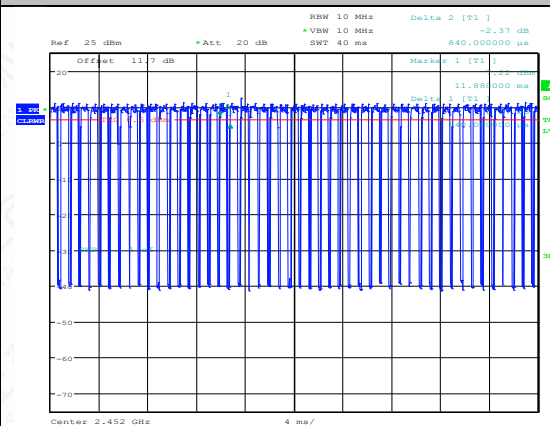
NTNV-11N40MIMO-Ant1-2452
