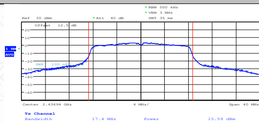
11G-CDD-Ant1-2437-PASS
