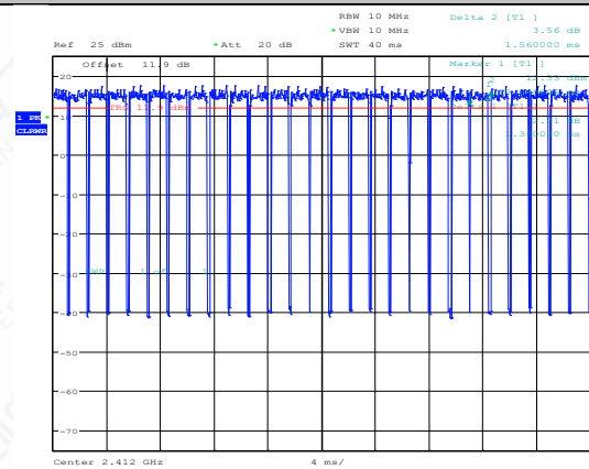
NTNV-11N20MIMO-Ant2-2412
