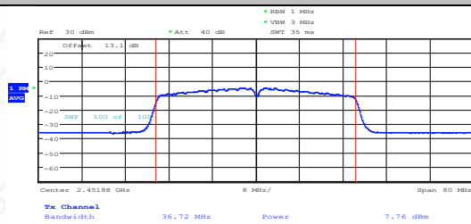
11N40SISO-Ant1-2452-PASS
