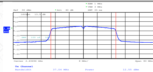
11N40SISO-Ant2-2437-PASS
