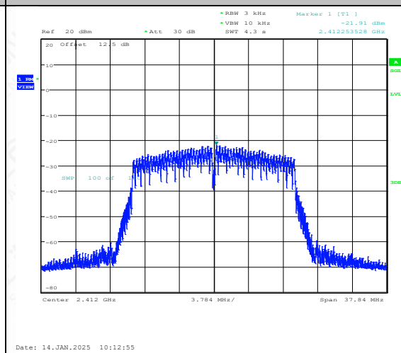
11N20MIMO-Ant2-2412-PASS
