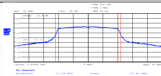
11G-CDD-Ant2-2437-PASS
