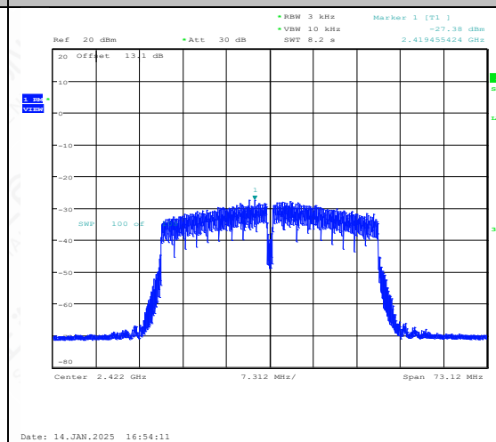
11N40SISO-Ant1-2422-PASS
