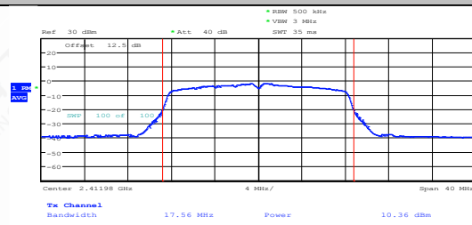
11G-CDD-Ant2-2412-PASS
