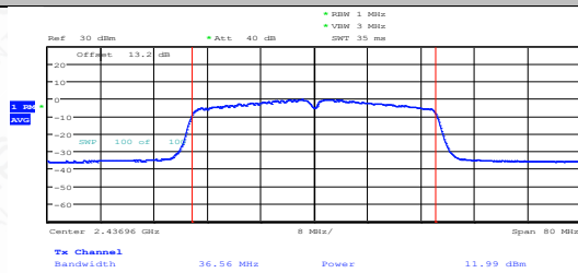
11N40SISO-Ant1-2437-PASS
