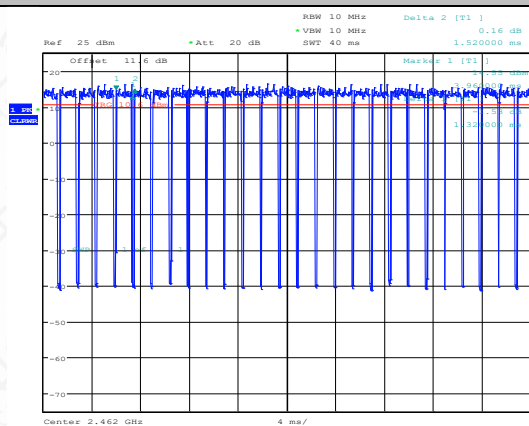
NTNV-11N20SISO-Ant1-2462
