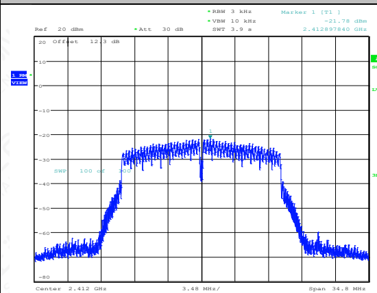
11G-Ant1-2412-PASS
