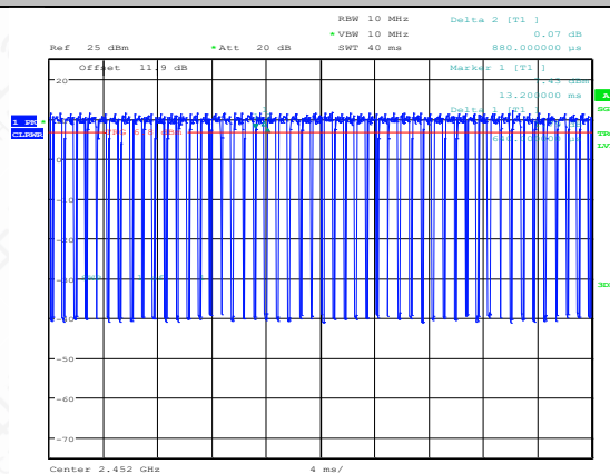
NTNV-11N40MIMO-Ant2-2452
