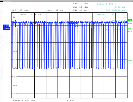
NTNV-11N40SISO-Ant1-2437
