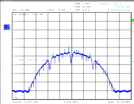
11B-CDD-Ant2-2437-PASS
