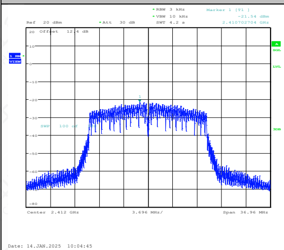
11N20MIMO-Ant1-2412-PASS
