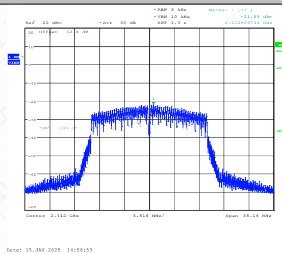
11N20SISO-Ant2-2412-PASS
