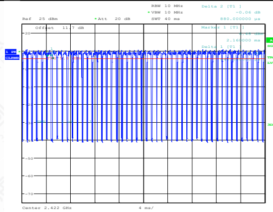
NTNV-11N40SISO-Ant1-2422
