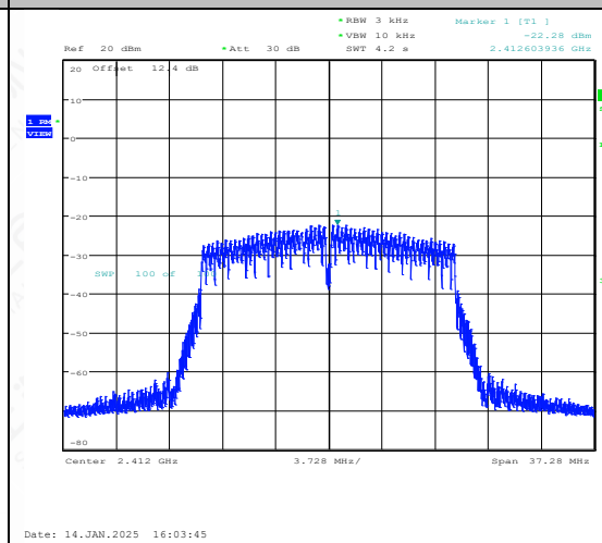
11N20SISO-Ant1-2412-PASS
