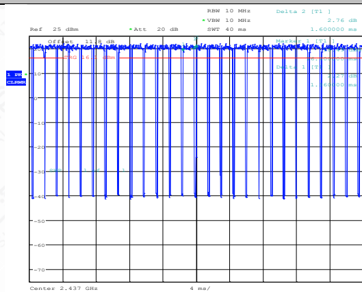
NTNV-11N20SISO-Ant1-2437
