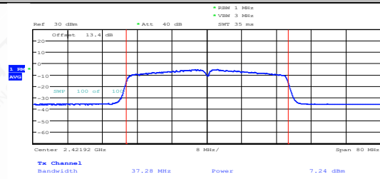
11N40SISO-Ant2-2422-PASS
