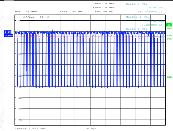
NTNV-11N40SISO-Ant2-2422
