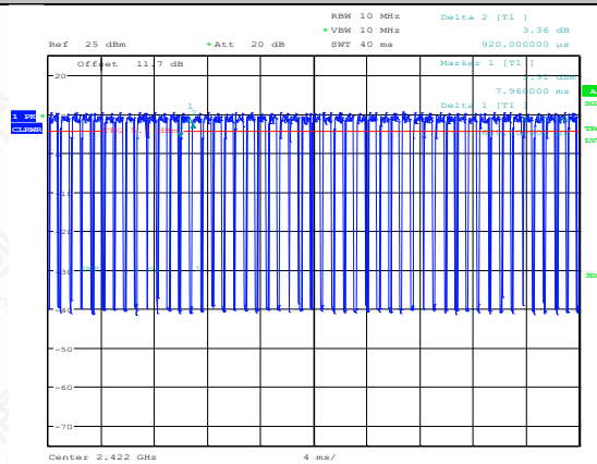
NTNV-11N40MIMO-Ant1-2422
