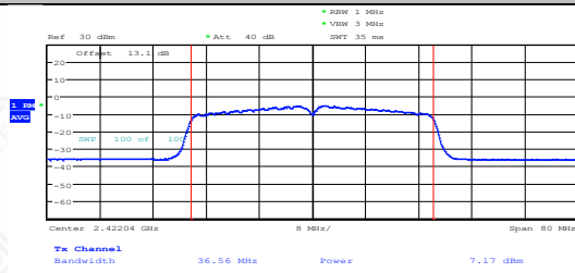
11N40SISO-Ant1-2422-PASS
