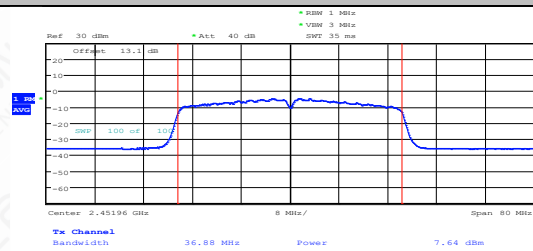
11N40SISO-Ant2-2452-PASS
