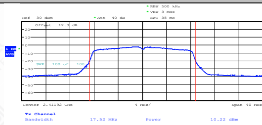
11G-CDD-Ant1-2412-PASS
