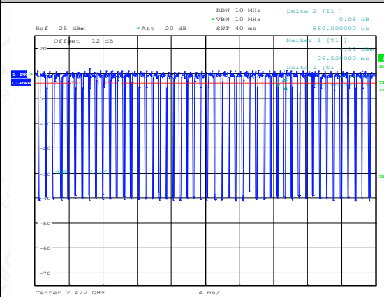
NTNV-11N40MIMO-Ant2-2422
