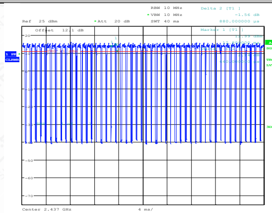
NTNV-11N40SISO-Ant2-2437
